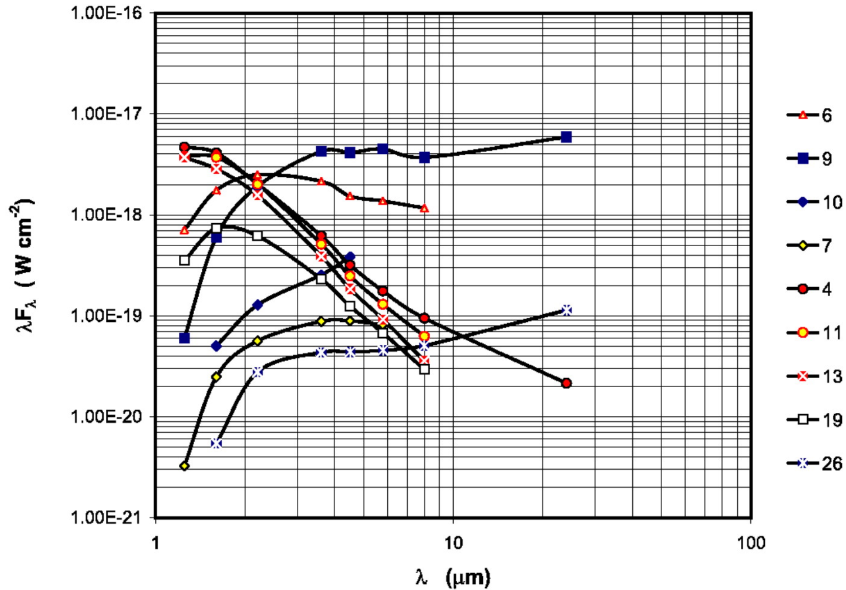
Fig. 6. from Spitzer and Magellan Observations of NGC 2264: A Remarkable Starforming Core near IRS 2 Young et al. 2006 ApJ 642 972 doi:10.1086/501227 https://dx.doi.org/10.1086/501227 © 2006. The American Astronomical Society. All rights reserved. Printed in U.S.A.
