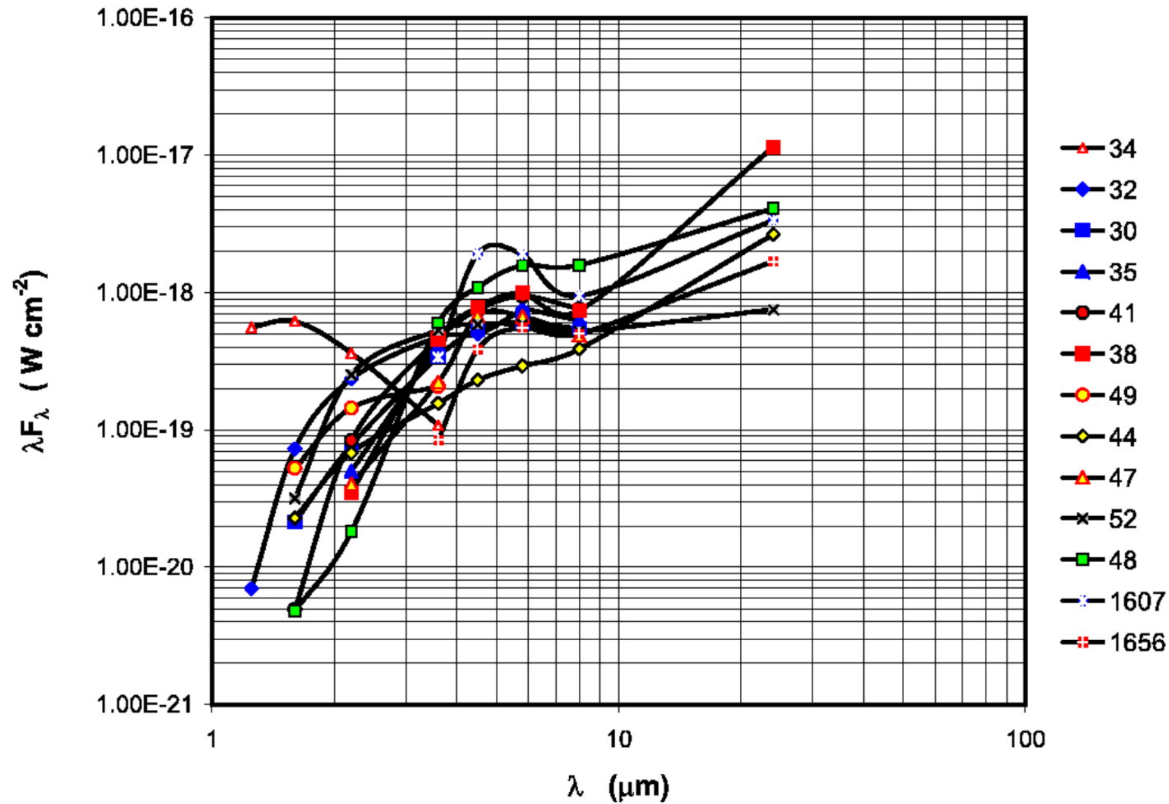
Fig. 5. from Spitzer and Magellan Observations of NGC 2264: A Remarkable Starforming Core near IRS 2 Young et al. 2006 ApJ 642 972 doi:10.1086/501227 https://dx.doi.org/10.1086/501227 © 2006. The American Astronomical Society. All rights reserved. Printed in U.S.A.
