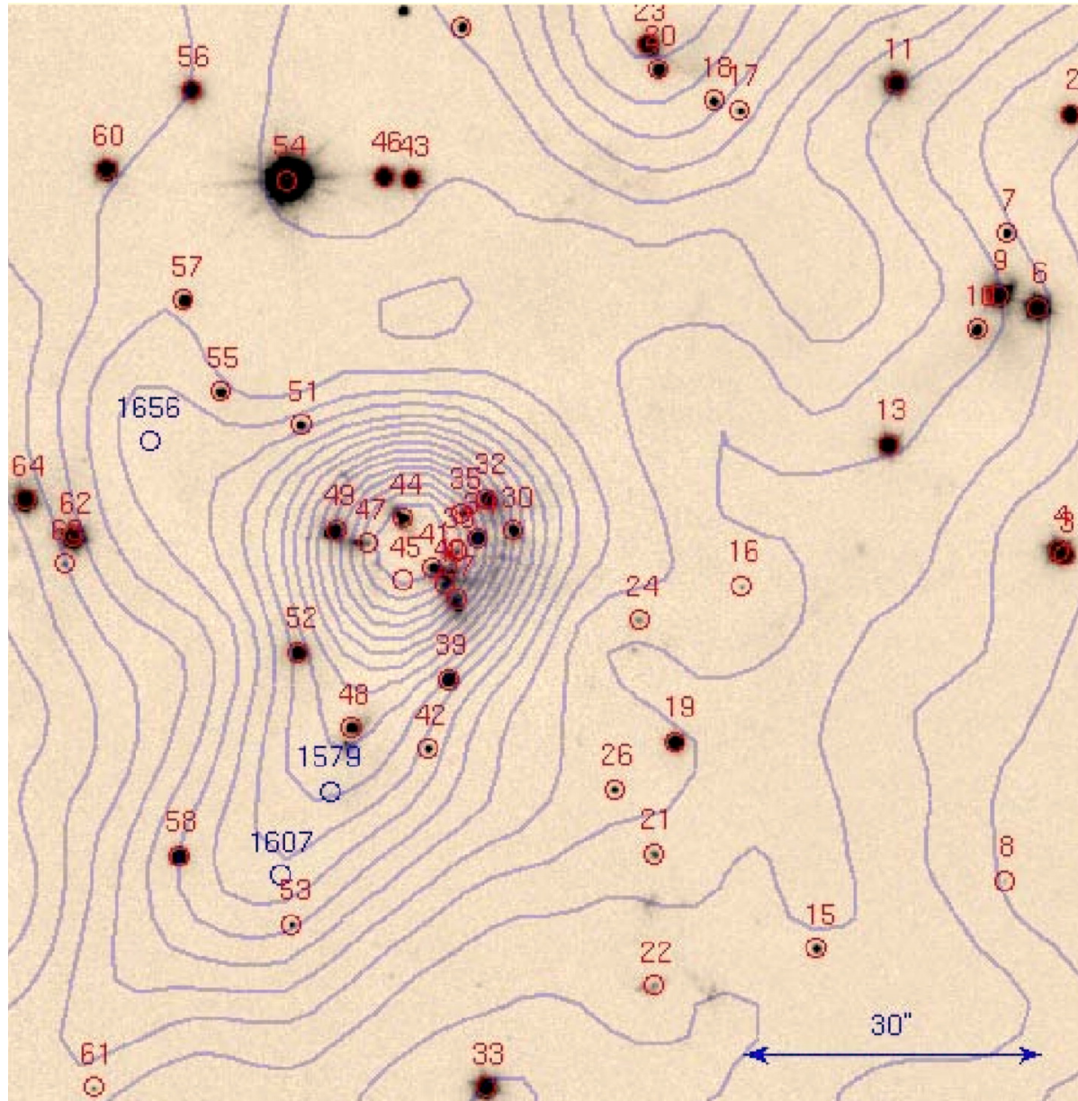
Fig. 4. from Spitzer and Magellan Observations of NGC 2264: A Remarkable Starforming Core near IRS 2 Young et al. 2006 ApJ 642 972 doi:10.1086/501227 https://dx.doi.org/10.1086/501227 © 2006. The American Astronomical Society. All rights reserved. Printed in U.S.A.
