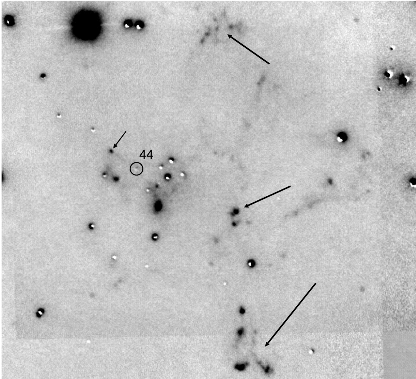
Fig. 3. from Spitzer and Magellan Observations of NGC 2264: A Remarkable Starforming Core near IRS 2 Young et al. 2006 ApJ 642 972 doi:10.1086/501227 https://dx.doi.org/10.1086/501227 © 2006. The American Astronomical Society. All rights reserved. Printed in U.S.A.
