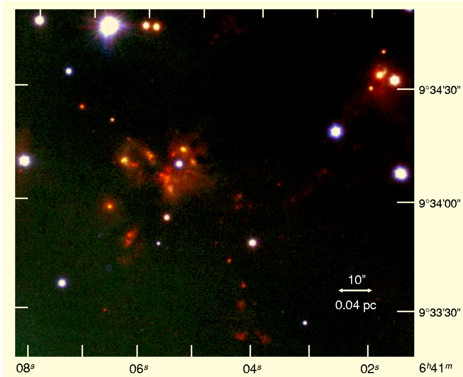
Fig. 2. from Spitzer and Magellan Observations of NGC 2264: A Remarkable Starforming Core near IRS 2 Young et al. 2006 ApJ 642 972 doi:10.1086/501227 https://dx.doi.org/10.1086/501227 © 2006. The American Astronomical Society. All rights reserved. Printed in U.S.A.
