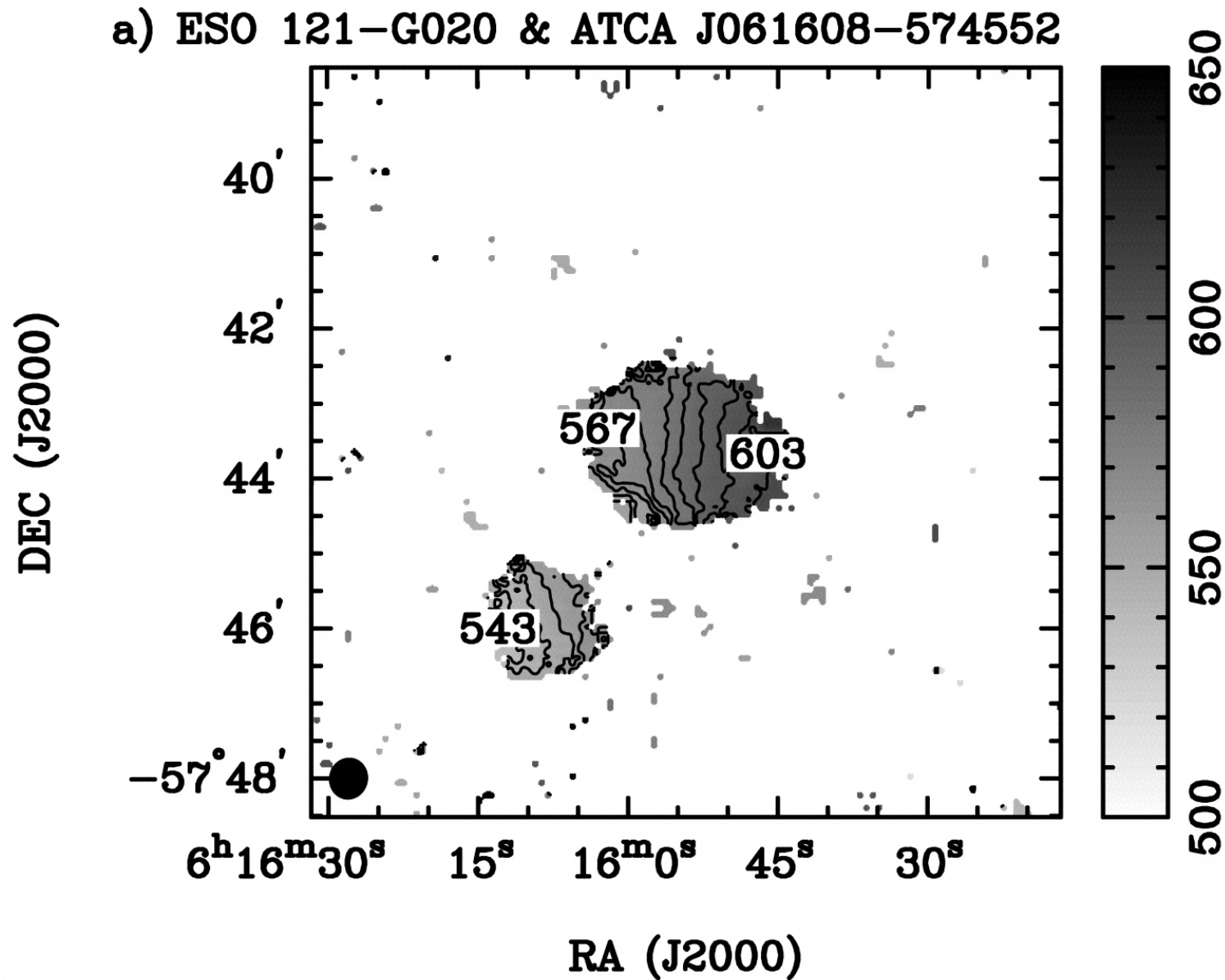
Fig. 7. from Stellar and Gas Properties of High H I MasstoLight Ratio Galaxies in the Local Universe Warren, Jerjen, & Koribalski 2006 AJ 131 2056 doi:10.1086/500589 https://dx.doi.org/10.1086/500589 © 2006. The American Astronomical Society. All rights reserved. Printed in U.S.A.
