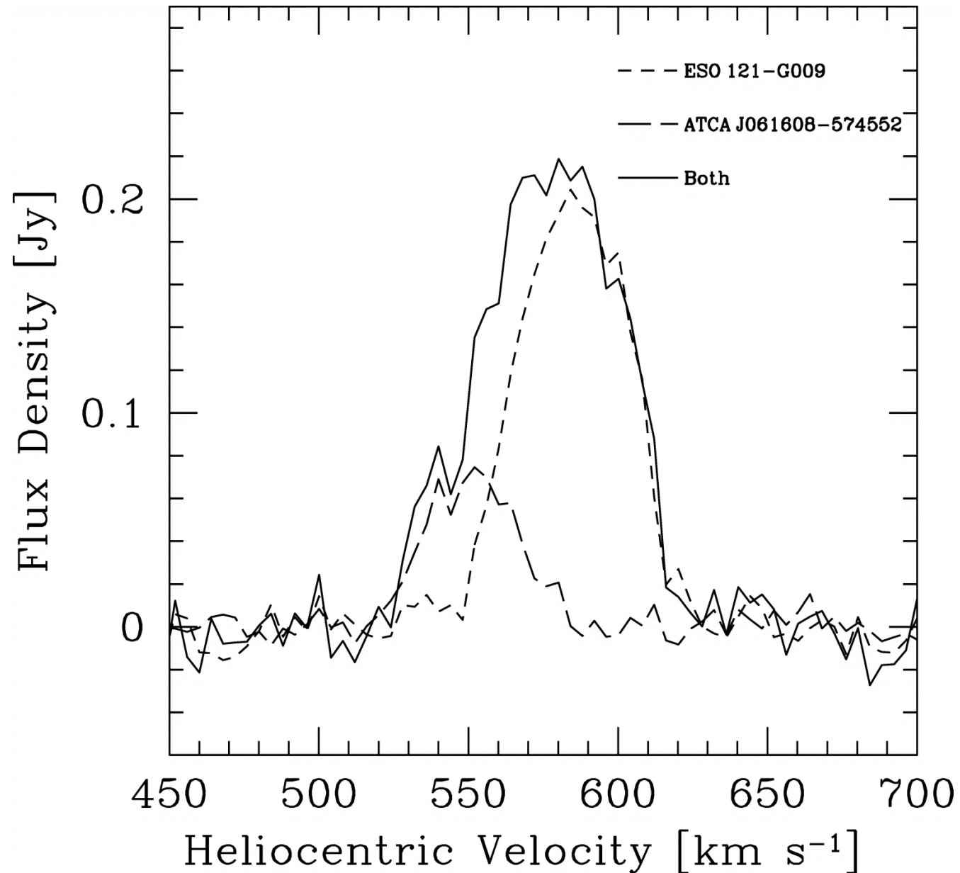
Fig. 6. from Stellar and Gas Properties of High H I MasstoLight Ratio Galaxies in the Local Universe Warren, Jerjen, & Koribalski 2006 AJ 131 2056 doi:10.1086/500589 https://dx.doi.org/10.1086/500589 © 2006. The American Astronomical Society. All rights reserved. Printed in U.S.A.
