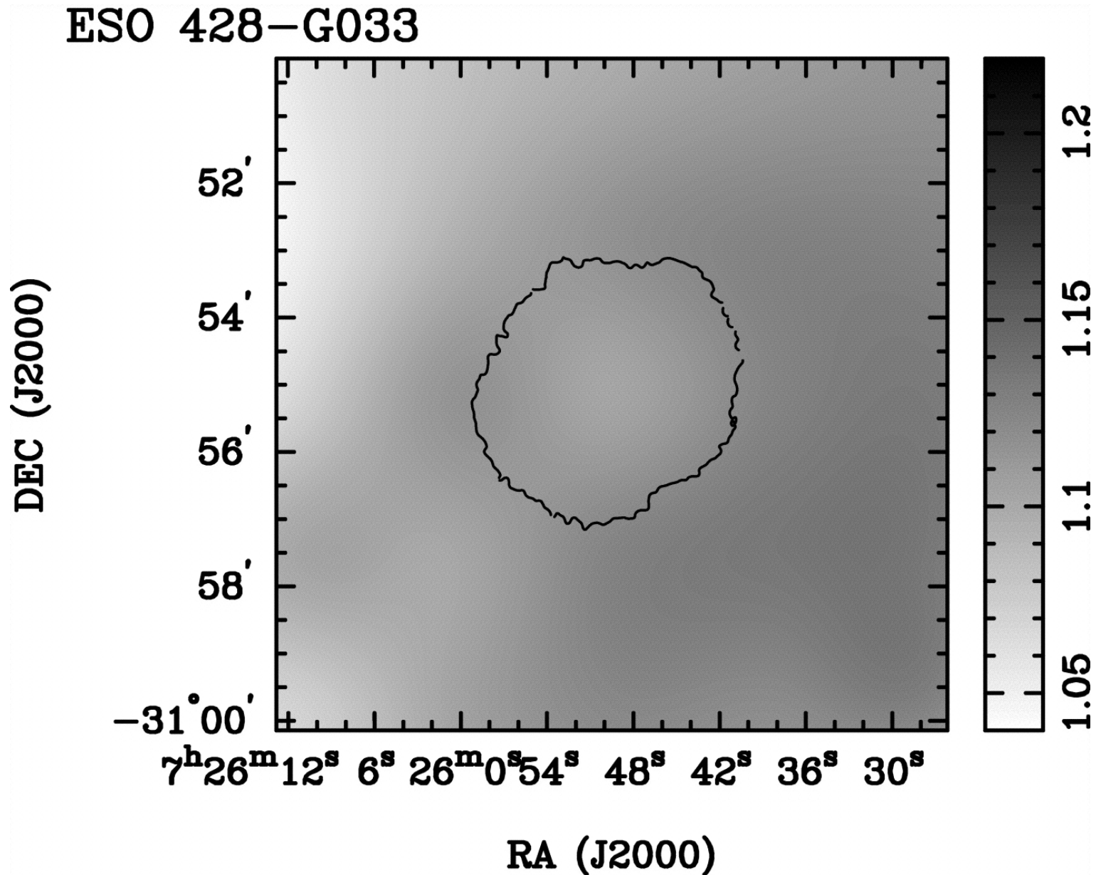
Fig. 12. from Stellar and Gas Properties of High H I MasstoLight Ratio Galaxies in the Local Universe Warren, Jerjen, & Koribalski 2006 AJ 131 2056 doi:10.1086/500589 https://dx.doi.org/10.1086/500589 © 2006. The American Astronomical Society. All rights reserved. Printed in U.S.A.
