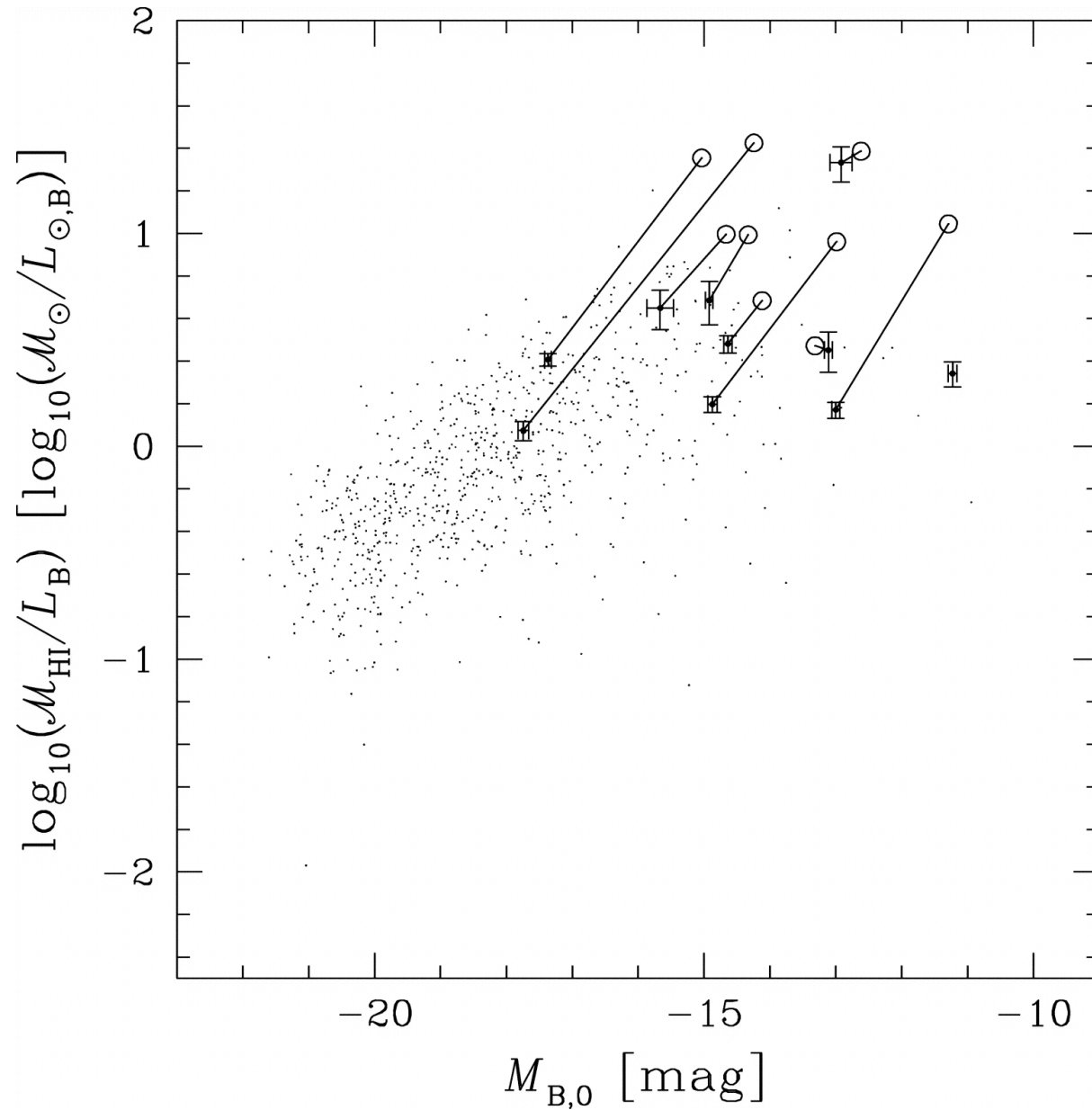
Fig. 11. from Stellar and Gas Properties of High H I MasstoLight Ratio Galaxies in the Local Universe Warren, Jerjen, & Koribalski 2006 AJ 131 2056 doi:10.1086/500589 https://dx.doi.org/10.1086/500589
