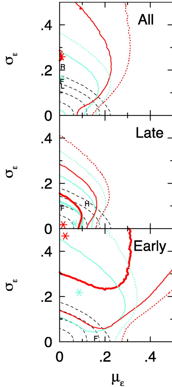
Fig. 7. from The Intrinsic Shape of Spiral Galaxies in the 2MASS Large Galaxy Atlas Ryden 2006 ApJ 641 773 doi:10.1086/500497 https://dx.doi.org/10.1086/500497 © 2006. The American Astronomical Society. All rights reserved. Printed in U.S.A.
