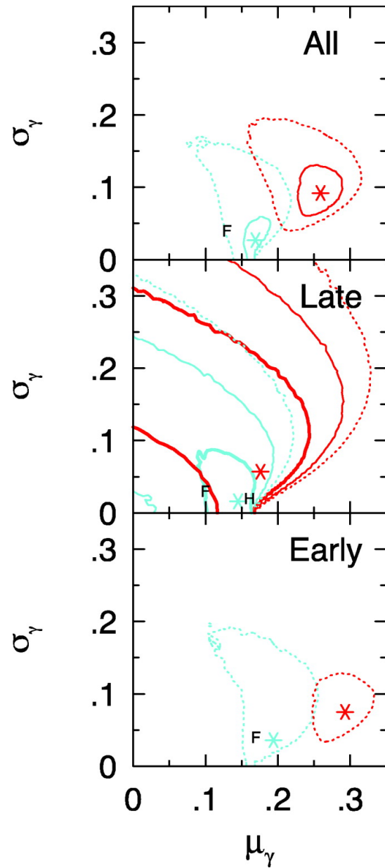
Fig. 6. from The Intrinsic Shape of Spiral Galaxies in the 2MASS Large Galaxy Atlas Ryden 2006 ApJ 641 773 doi:10.1086/500497 https://dx.doi.org/10.1086/500497 © 2006. The American Astronomical Society. All rights reserved. Printed in U.S.A.
