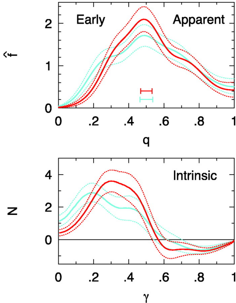
Fig. 5. from The Intrinsic Shape of Spiral Galaxies in the 2MASS Large Galaxy Atlas Ryden 2006 ApJ 641 773 doi:10.1086/500497 https://dx.doi.org/10.1086/500497 © 2006. The American Astronomical Society. All rights reserved. Printed in U.S.A.
