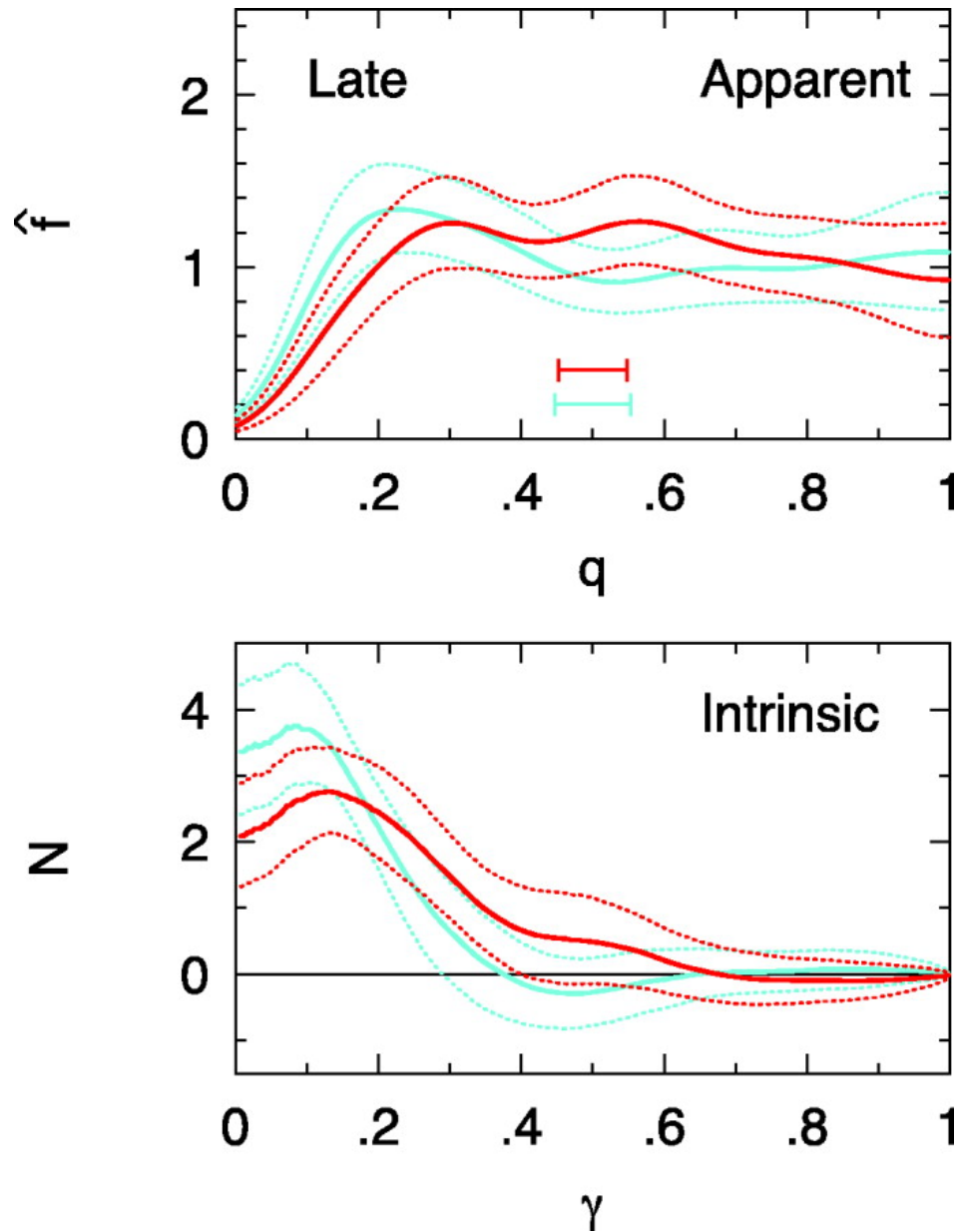
Fig. 4. from The Intrinsic Shape of Spiral Galaxies in the 2MASS Large Galaxy Atlas Ryden 2006 ApJ 641 773 doi:10.1086/500497 https://dx.doi.org/10.1086/500497 © 2006. The American Astronomical Society. All rights reserved. Printed in U.S.A.
