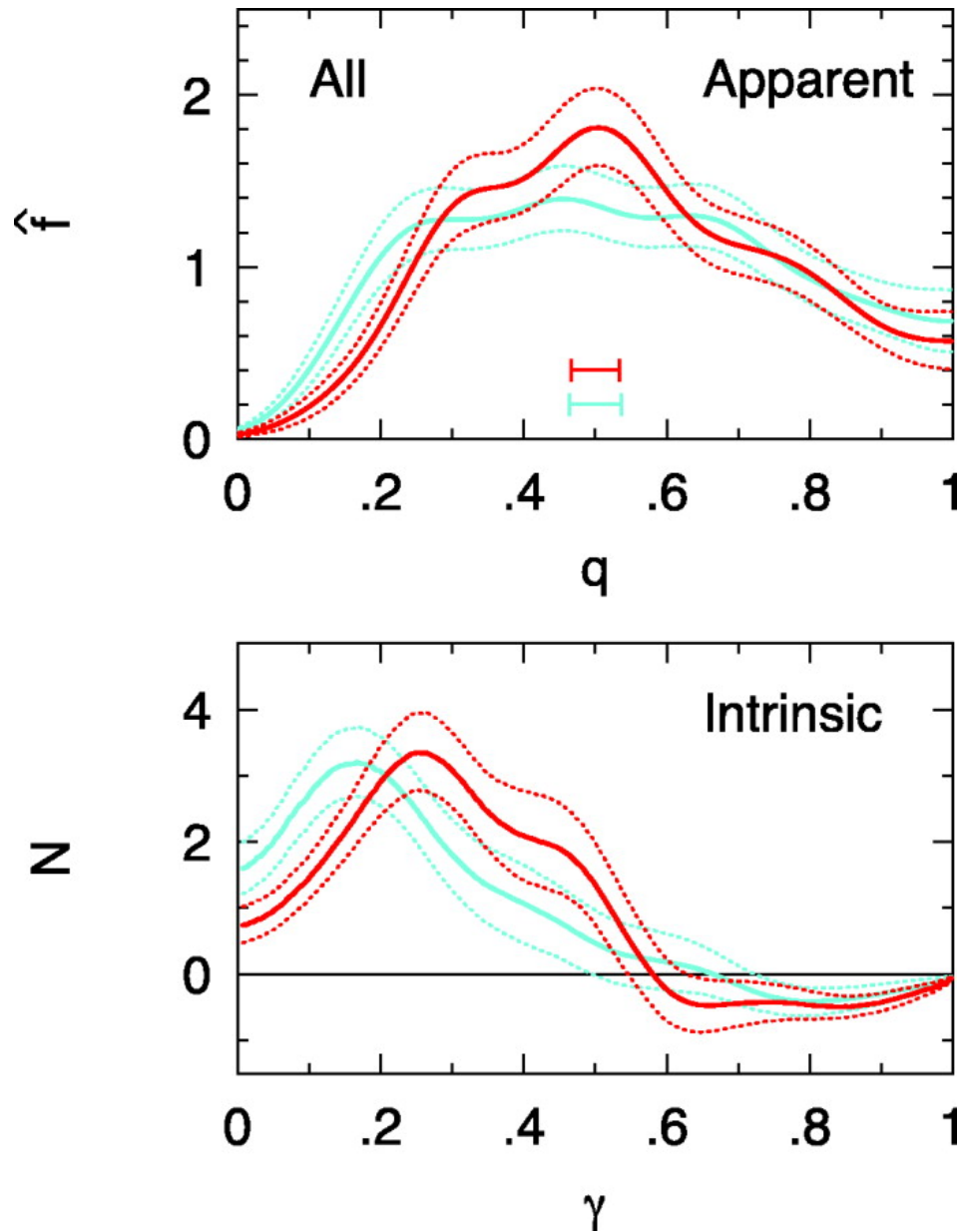
Fig. 3. from The Intrinsic Shape of Spiral Galaxies in the 2MASS Large Galaxy Atlas Ryden 2006 ApJ 641 773 doi:10.1086/500497 https://dx.doi.org/10.1086/500497 © 2006. The American Astronomical Society. All rights reserved. Printed in U.S.A.
