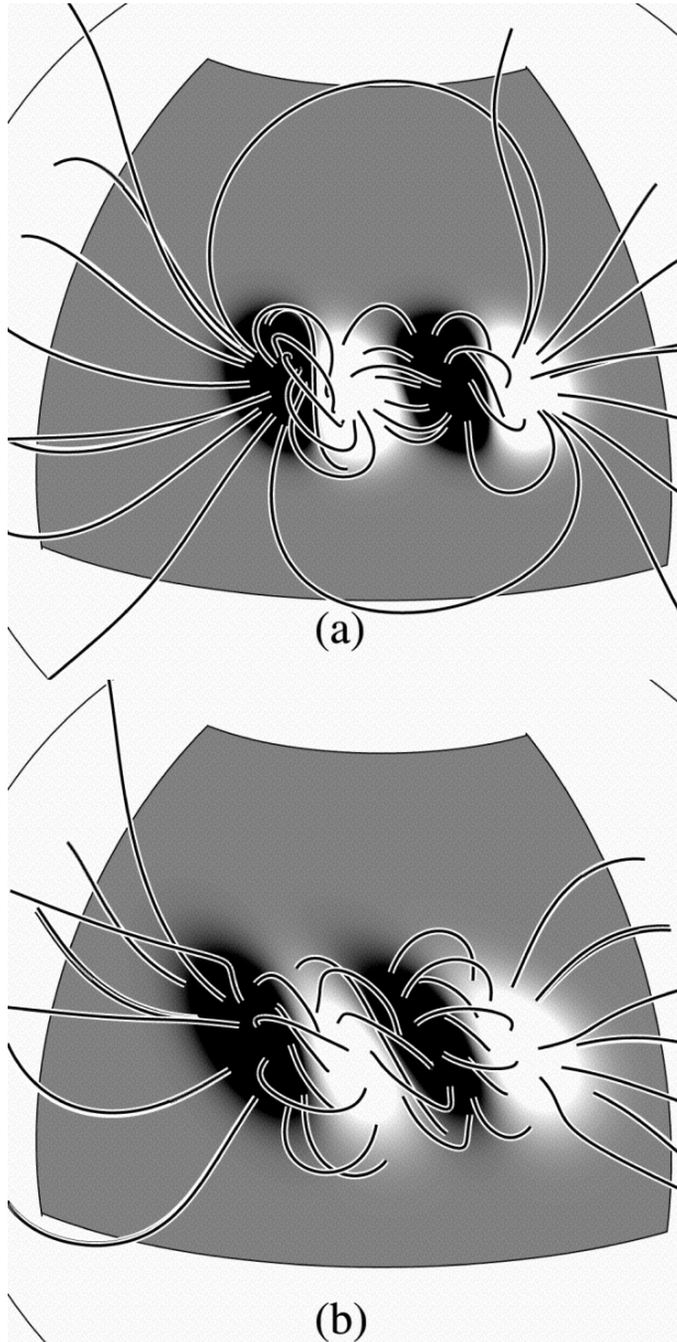
Fig. 5. from Models of the LargeScale Corona. I. Formation, Evolution, and Liftoff of Magnetic Flux Ropes Mackay & van Ballegoijen 2006 ApJ 641 577 doi:10.1086/500425 https://dx.doi.org/10.1086/500425
