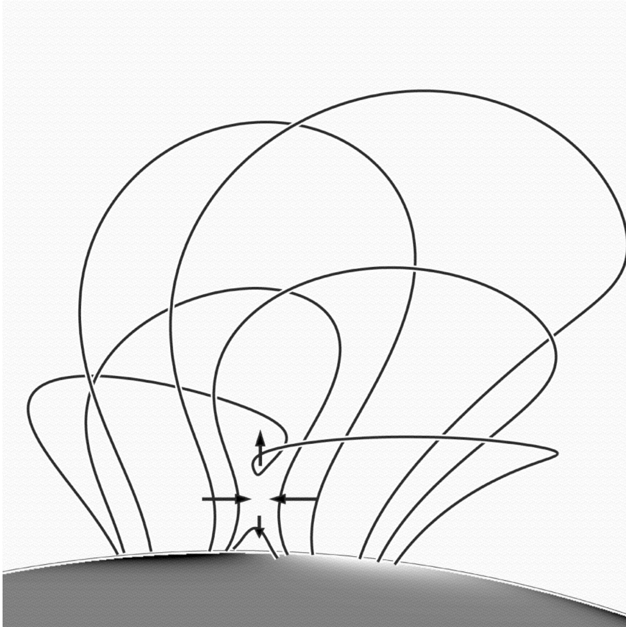
Fig. 12. from Models of the LargeScale Corona. I. Formation, Evolution, and Liftoff of Magnetic Flux Ropes Mackay & van Ballegoijen 2006 ApJ 641 577 doi:10.1086/500425 https://dx.doi.org/10.1086/500425 © 2006. The American Astronomical Society. All rights reserved. Printed in U.S.A.
