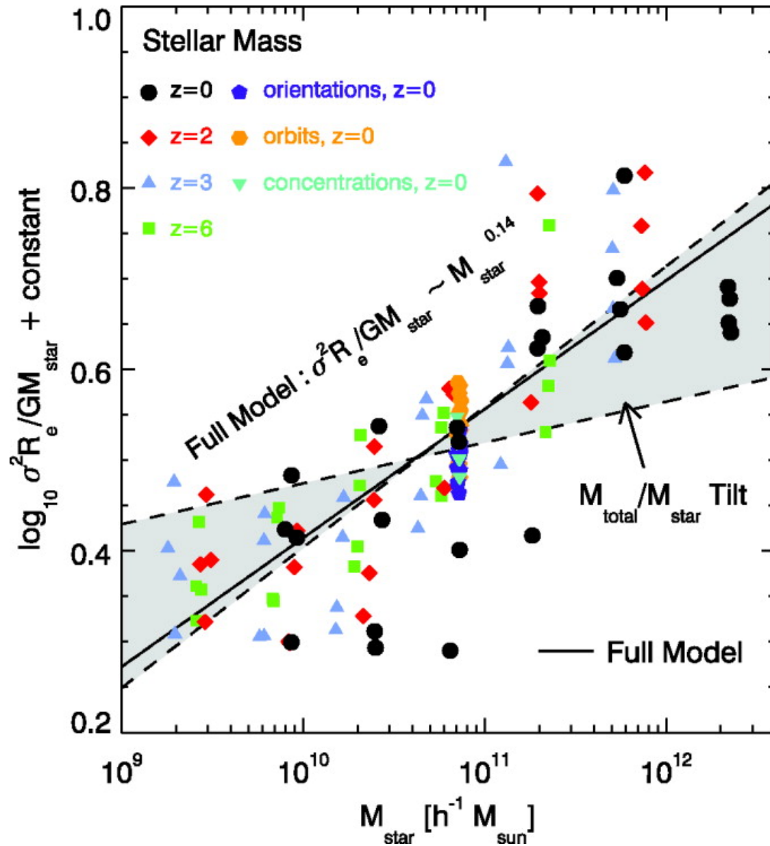
Fig. 16. from The Fundamental Scaling Relations of Elliptical Galaxies Robertson et al. 2006 ApJ 641 21 doi:10.1086/500360 https://dx.doi.org/10.1086/500360 © 2006. The American Astronomical Society. All rights reserved. Printed in U.S.A.
