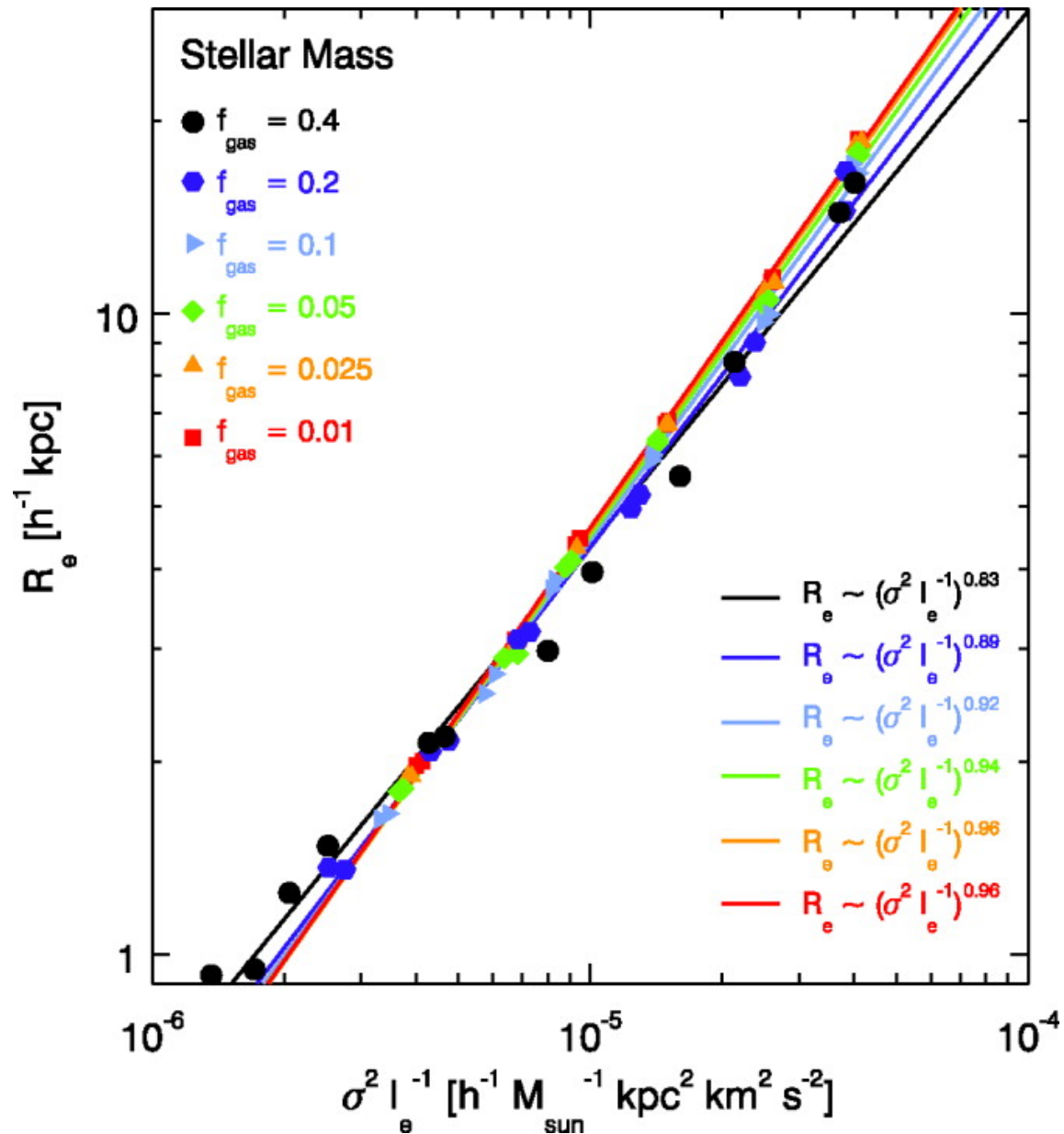
Fig. 10. from The Fundamental Scaling Relations of Elliptical Galaxies Robertson et al. 2006 ApJ 641 21 doi:10.1086/500360 https://dx.doi.org/10.1086/500360 © 2006. The American Astronomical Society. All rights reserved. Printed in U.S.A.
