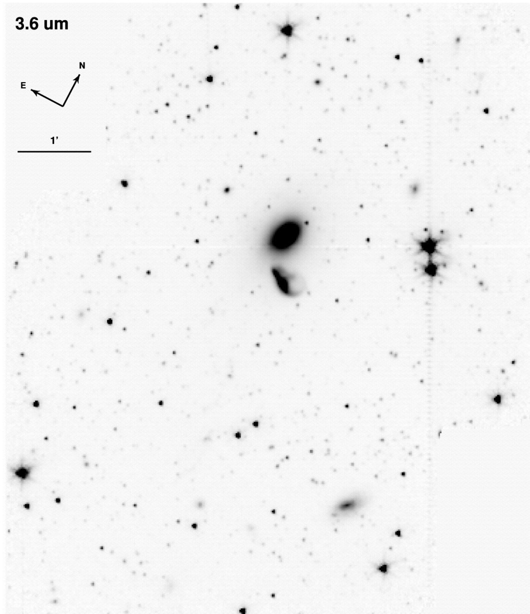
Fig. 9. from First Detection of PAHs and Warm Molecular Hydrogen in Tidal Dwarf Galaxies Higdon, Higdon, & Marshall 2006 ApJ 640 768 doi:10.1086/500254 https://dx.doi.org/10.1086/500254
