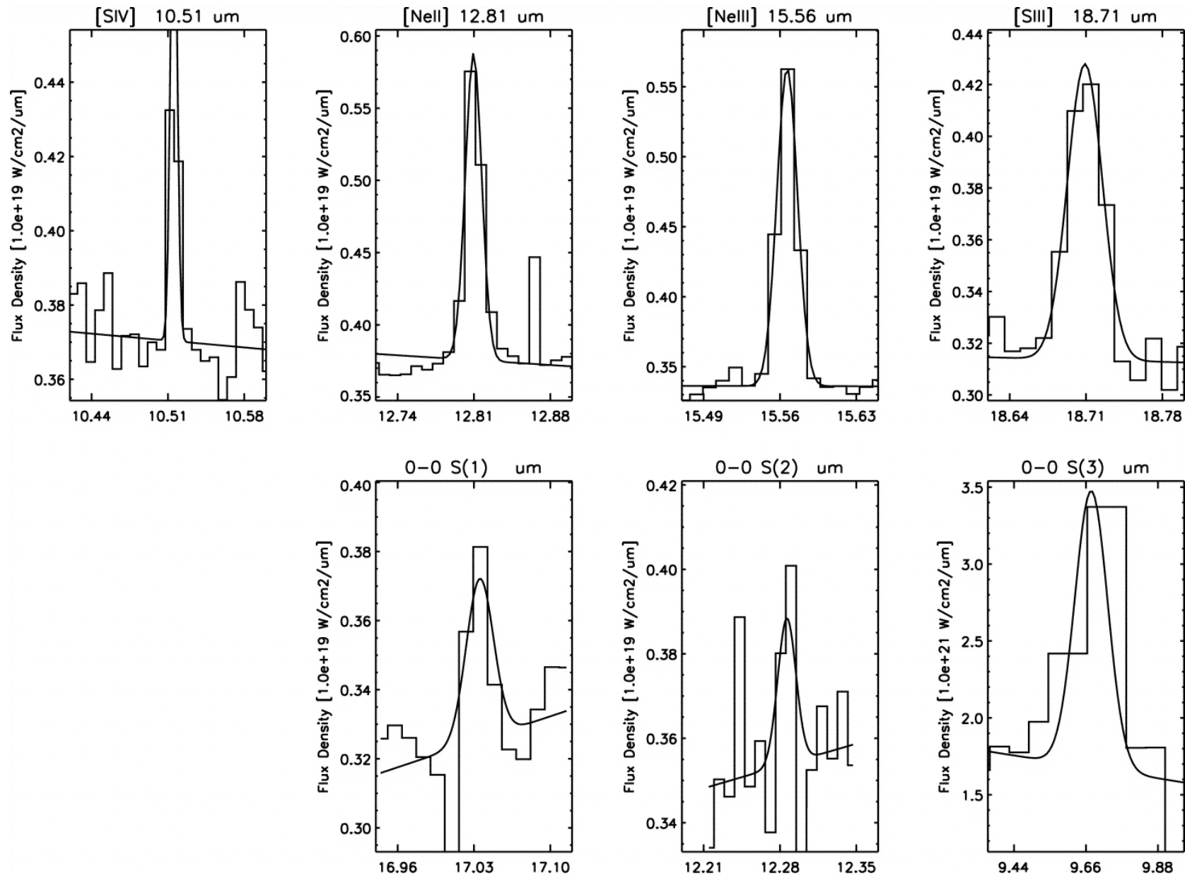
Fig. 6. from First Detection of PAHs and Warm Molecular Hydrogen in Tidal Dwarf Galaxies Higdon, Higdon, & Marshall 2006 ApJ 640 768 doi:10.1086/500254 https://dx.doi.org/10.1086/500254
