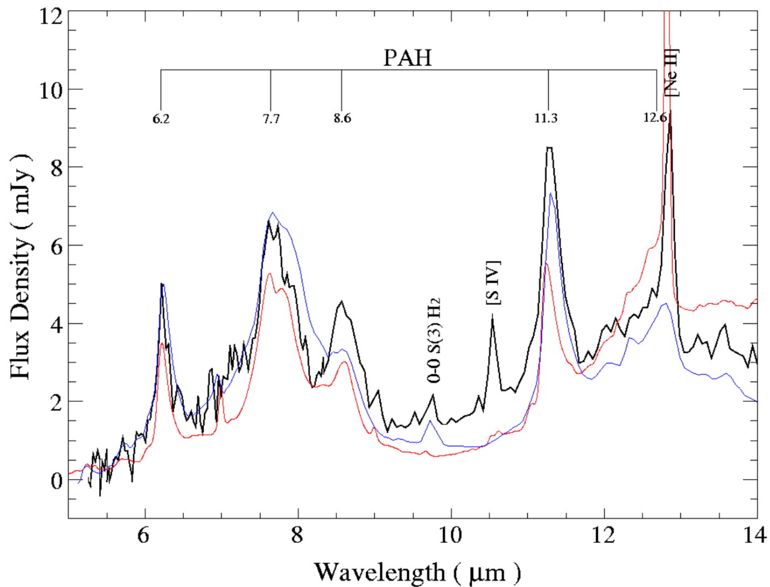
Fig. 4. from First Detection of PAHs and Warm Molecular Hydrogen in Tidal Dwarf Galaxies Higdon, Higdon, & Marshall 2006 ApJ 640 768 doi:10.1086/500254 https://dx.doi.org/10.1086/500254 © 2006. The American Astronomical Society. All rights reserved. Printed in U.S.A.
