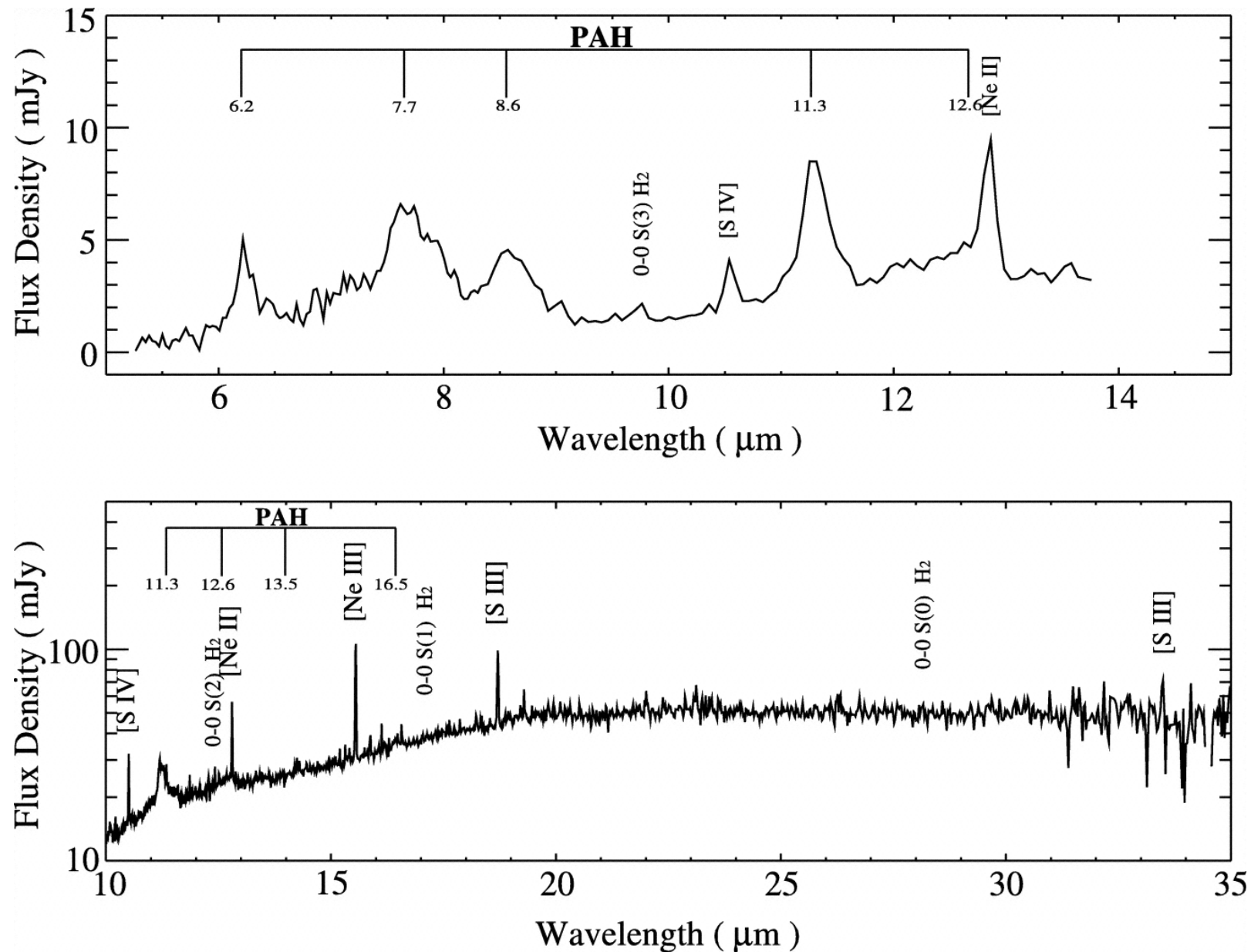
Fig. 2. from First Detection of PAHs and Warm Molecular Hydrogen in Tidal Dwarf Galaxies Higdon, Higdon, & Marshall 2006 ApJ 640 768 doi:10.1086/500254 https://dx.doi.org/10.1086/500254
