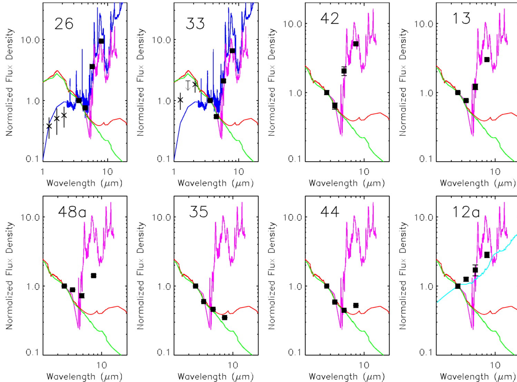
Fig. 12. from First Detection of PAHs and Warm Molecular Hydrogen in Tidal Dwarf Galaxies Higdon, Higdon, & Marshall 2006 ApJ 640 768 doi:10.1086/500254 https://dx.doi.org/10.1086/500254
