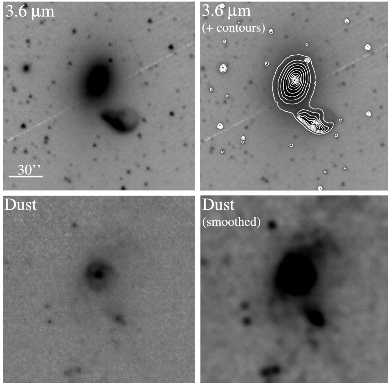
Fig. 11. from First Detection of PAHs and Warm Molecular Hydrogen in Tidal Dwarf Galaxies Higdon, Higdon, & Marshall 2006 ApJ 640 768 doi:10.1086/500254 https://dx.doi.org/10.1086/500254
