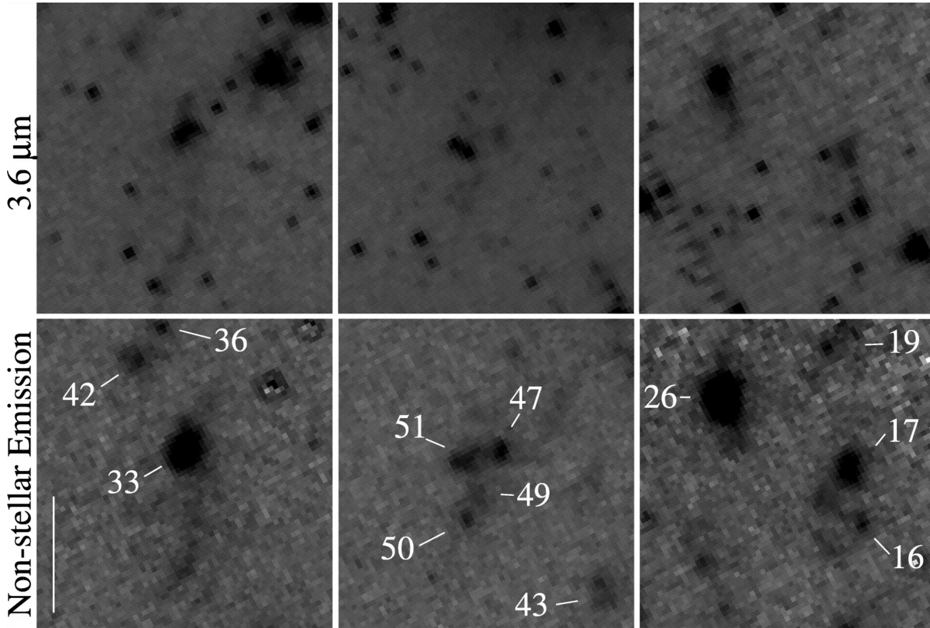
Fig. 10. from First Detection of PAHs and Warm Molecular Hydrogen in Tidal Dwarf Galaxies Higdon, Higdon, & Marshall 2006 ApJ 640 768 doi:10.1086/500254 https://dx.doi.org/10.1086/500254 © 2006. The American Astronomical Society. All rights reserved. Printed in U.S.A.
