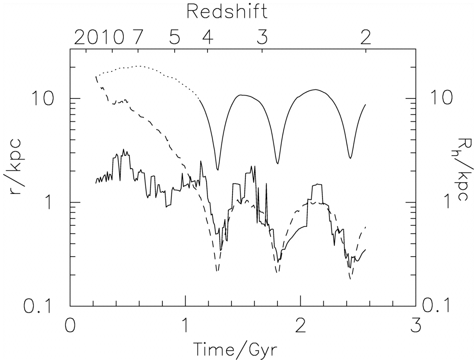
Fig. 7. from Tidal Disruption of Dark Matter Halos around Proto-Globular Clusters Saitoh et al. 2006 ApJ 640 22 doi:10.1086/500104 https://dx.doi.org/10.1086/500104 © 2006. The American Astronomical Society. All rights reserved. Printed in U.S.A.
