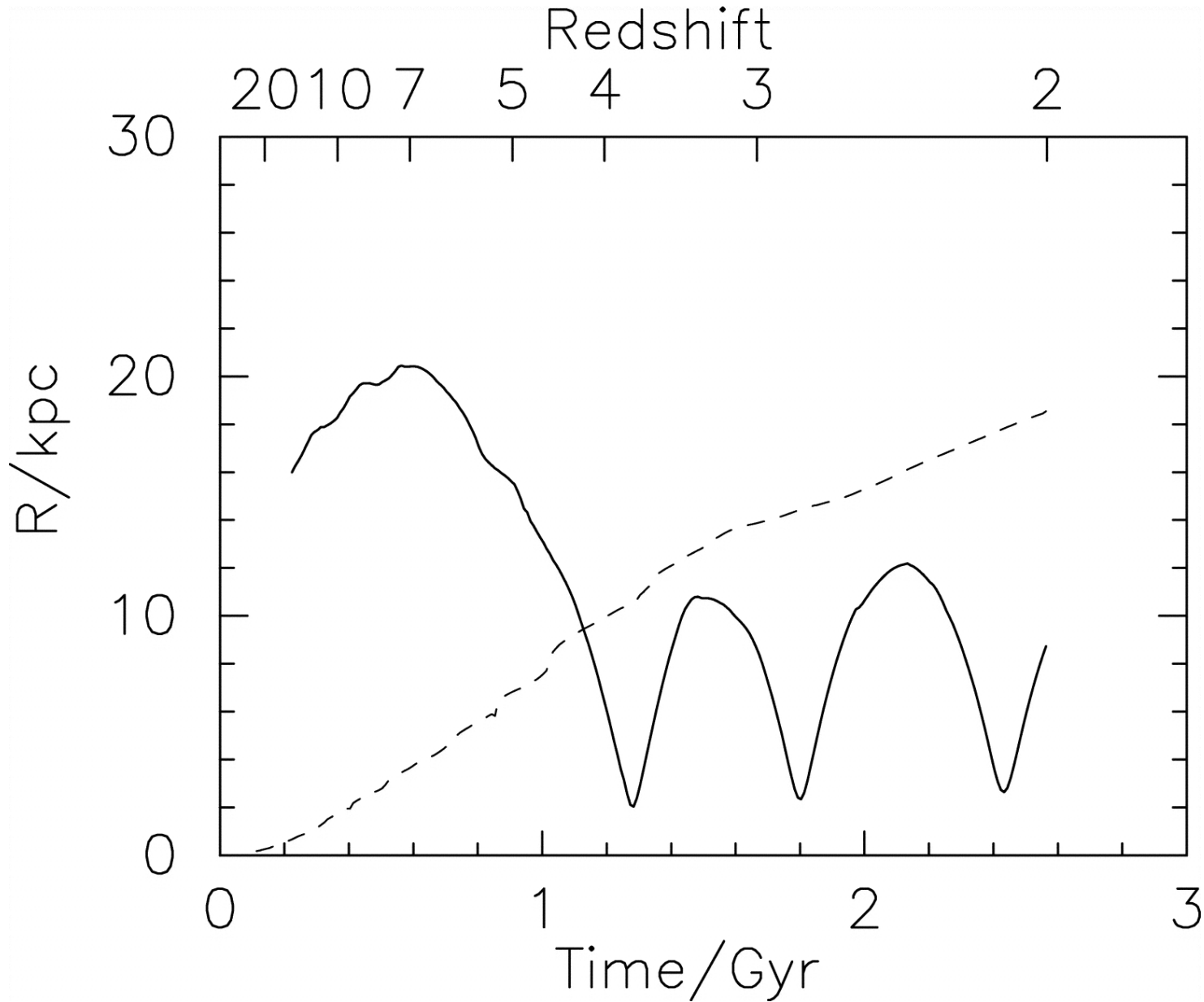
Fig. 6. from Tidal Disruption of Dark Matter Halos around Proto-Globular Clusters Saitoh et al. 2006 ApJ 640 22 doi:10.1086/500104 https://dx.doi.org/10.1086/500104 © 2006. The American Astronomical Society. All rights reserved. Printed in U.S.A.
