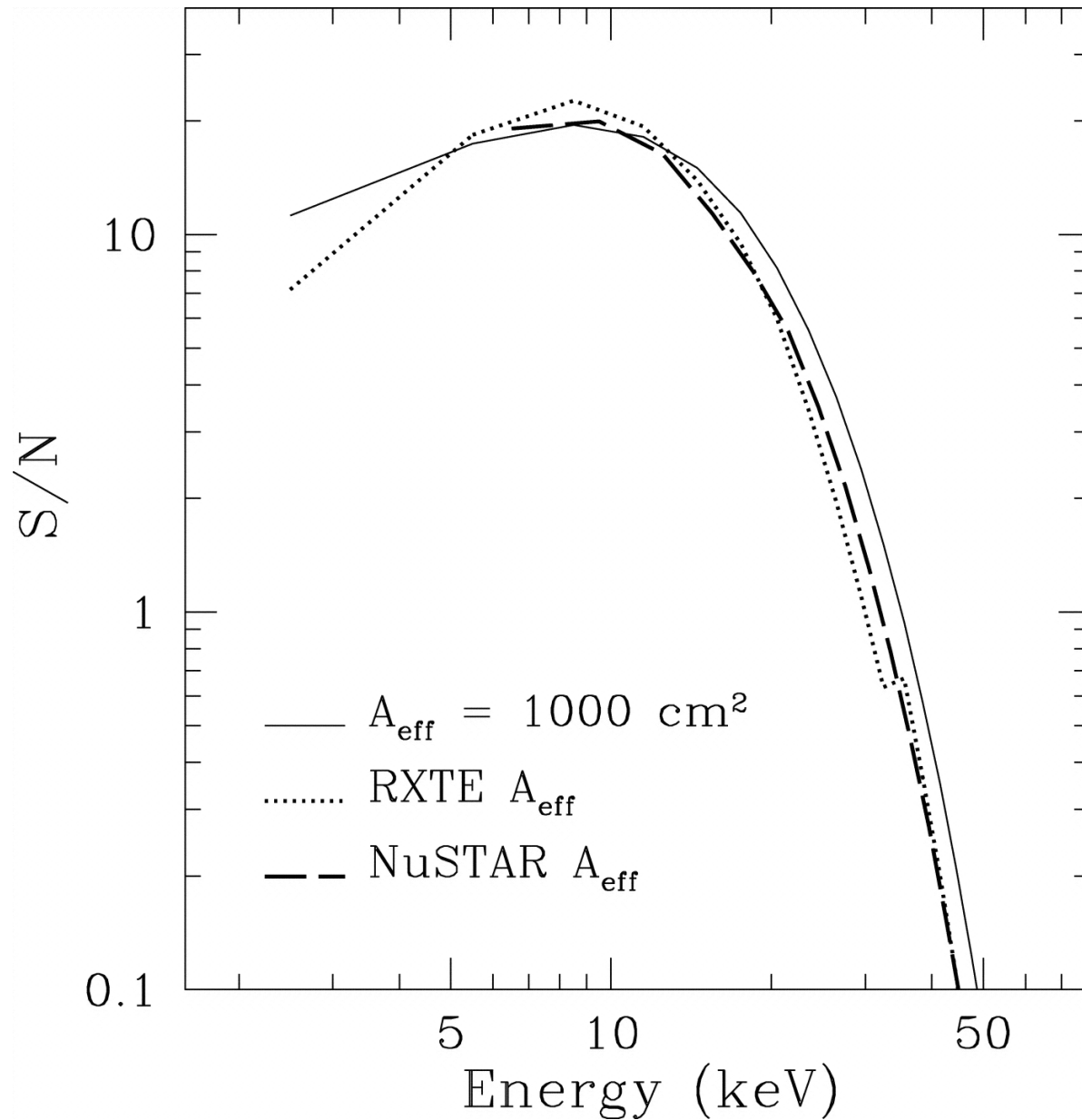
Fig. 5. from The Energy Dependence of Neutron Star Surface Modes and XRay Burst Oscillations Piro & Bildsten 2006 ApJ 638 968 doi:10.1086/499035 https://dx.doi.org/10.1086/499035 © 2006. The American Astronomical Society. All rights reserved. Printed in U.S.A.
