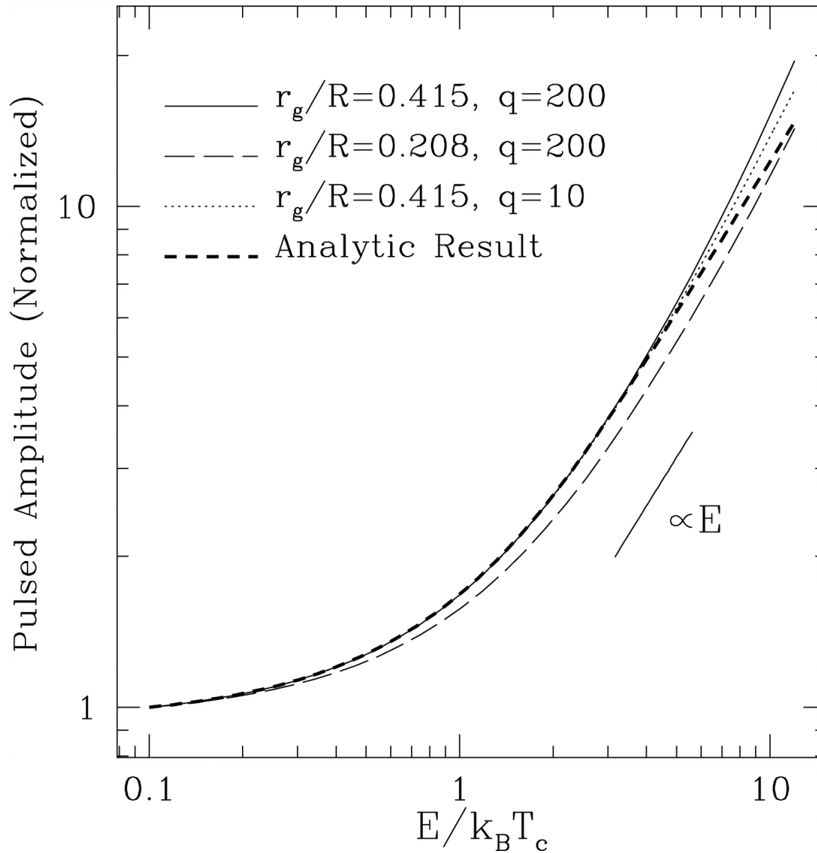
Fig. 2. from The Energy Dependence of Neutron Star Surface Modes and XRay Burst Oscillations Piro & Bildsten 2006 ApJ 638 968 doi:10.1086/499035 https://dx.doi.org/10.1086/499035 © 2006. The American Astronomical Society. All rights reserved. Printed in U.S.A.
