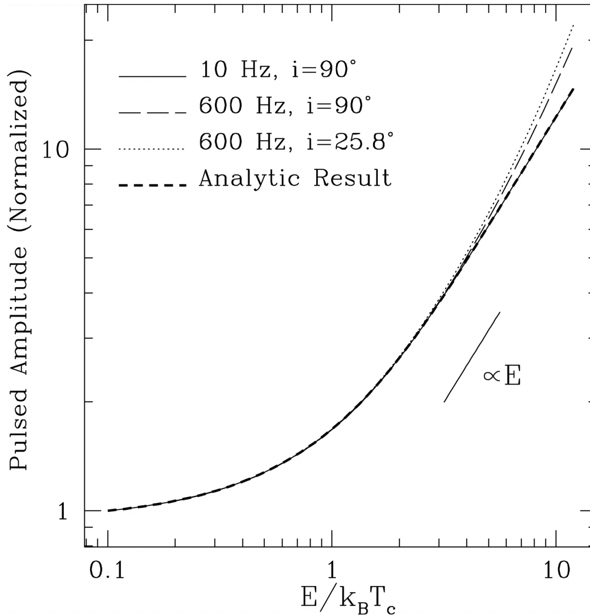
Fig. 1. from The Energy Dependence of Neutron Star Surface Modes and XRay Burst Oscillations Piro & Bildsten 2006 ApJ 638 968 doi:10.1086/499035 https://dx.doi.org/10.1086/499035 © 2006. The American Astronomical Society. All rights reserved. Printed in U.S.A.
