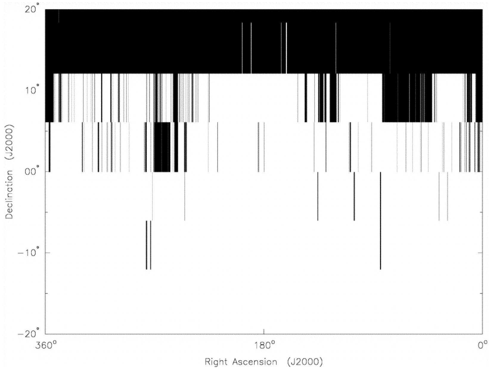
Fig. 9. from The Two Micron All Sky Survey (2MASS) Skrutskie et al. 2006 AJ 131 1163 doi:10.1086/498708 https://dx.doi.org/10.1086/498708
