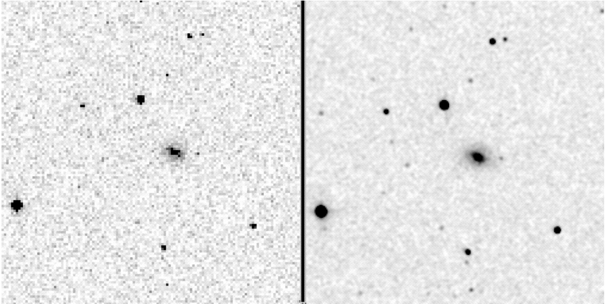
Fig. 8. from The Two Micron All Sky Survey (2MASS) Skrutskie et al. 2006 AJ 131 1163 doi:10.1086/498708 https://dx.doi.org/10.1086/498708
