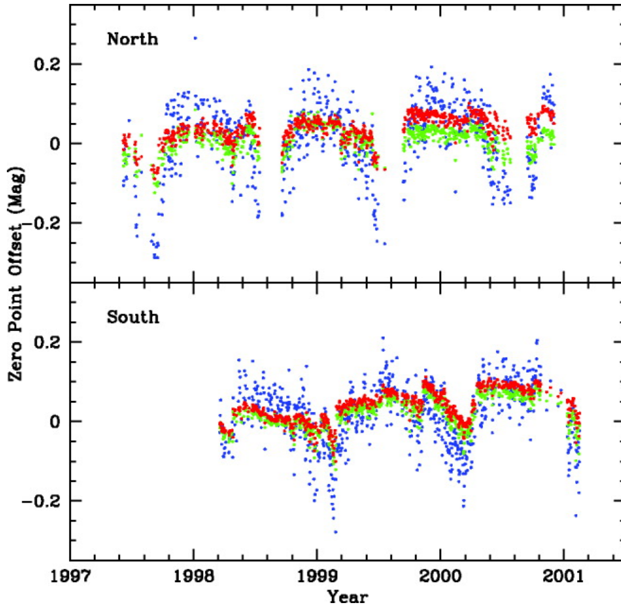
Fig. 7. from The Two Micron All Sky Survey (2MASS) Skrutskie et al. 2006 AJ 131 1163 doi:10.1086/498708 https://dx.doi.org/10.1086/498708
