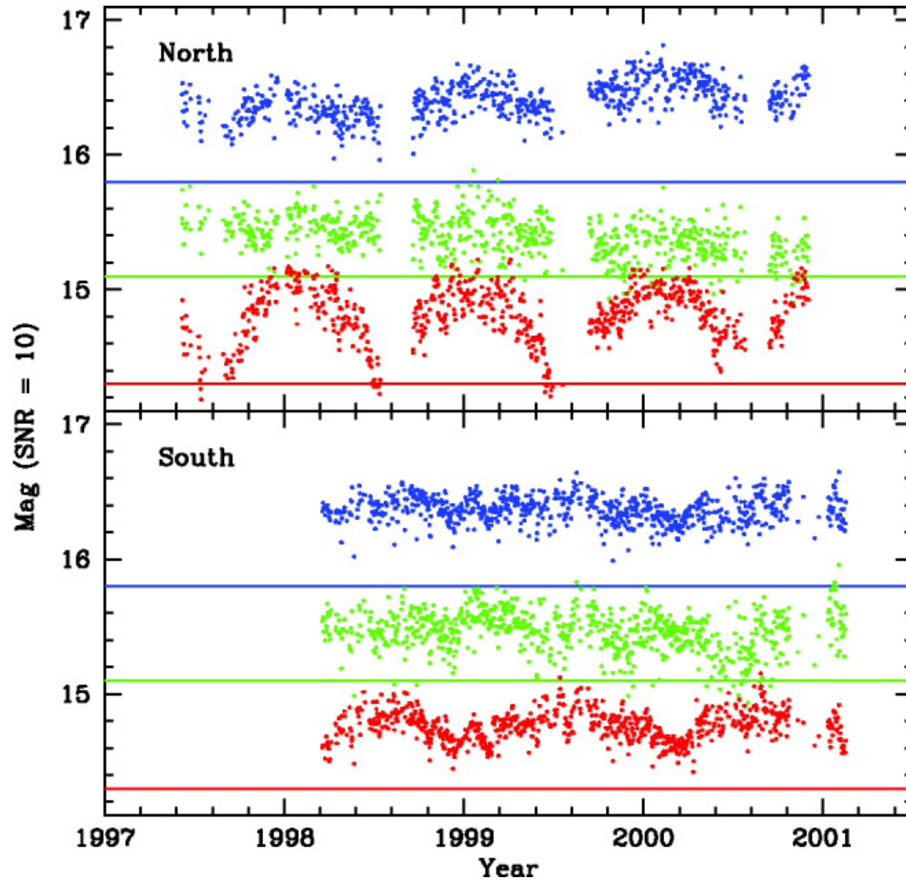
Fig. 6. from The Two Micron All Sky Survey (2MASS) Skrutskie et al. 2006 AJ 131 1163 doi:10.1086/498708 https://dx.doi.org/10.1086/498708
