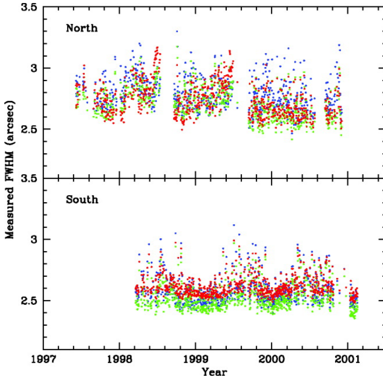
Fig. 5. from The Two Micron All Sky Survey (2MASS) Skrutskie et al. 2006 AJ 131 1163 doi:10.1086/498708 https://dx.doi.org/10.1086/498708
