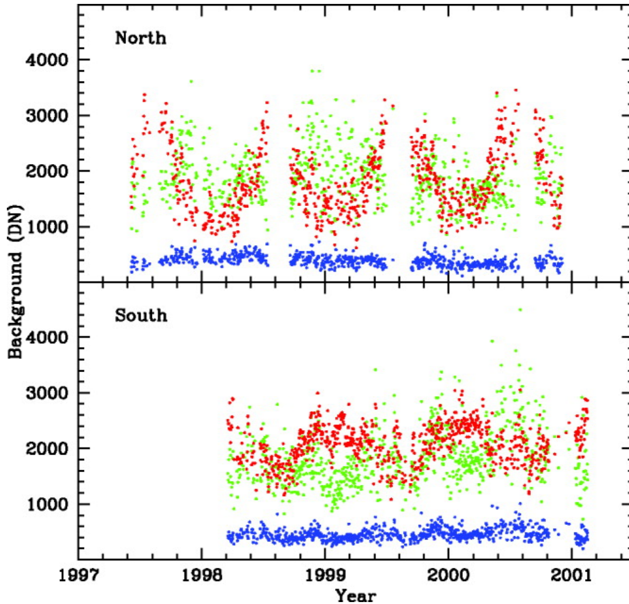
Fig. 4. from The Two Micron All Sky Survey (2MASS) Skrutskie et al. 2006 AJ 131 1163 doi:10.1086/498708 https://dx.doi.org/10.1086/498708
