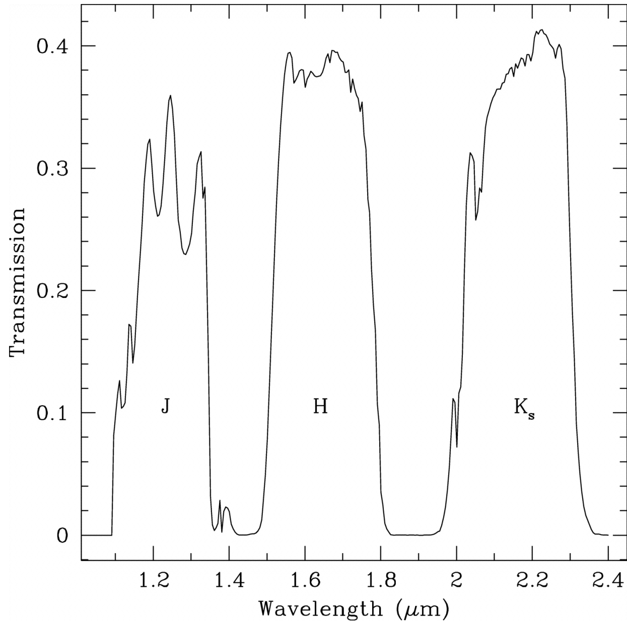
Fig. 2. from The Two Micron All Sky Survey (2MASS) Skrutskie et al. 2006 AJ 131 1163 doi:10.1086/498708 https://dx.doi.org/10.1086/498708
