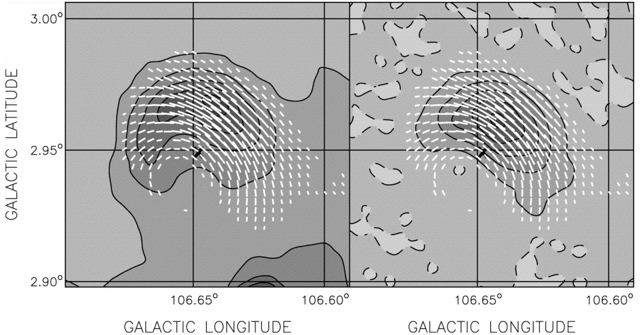
Fig. 7. from The Boomerang PWN G106.6+2.9 and the Magnetic Field Structure in Pulsar Wind Nebulae Kothes, Reich, & Uyanker 2006 ApJ 638 225 doi:10.1086/498666 https://dx.doi.org/10.1086/498666 © 2006. The American Astronomical Society. All rights reserved. Printed in U.S.A.
