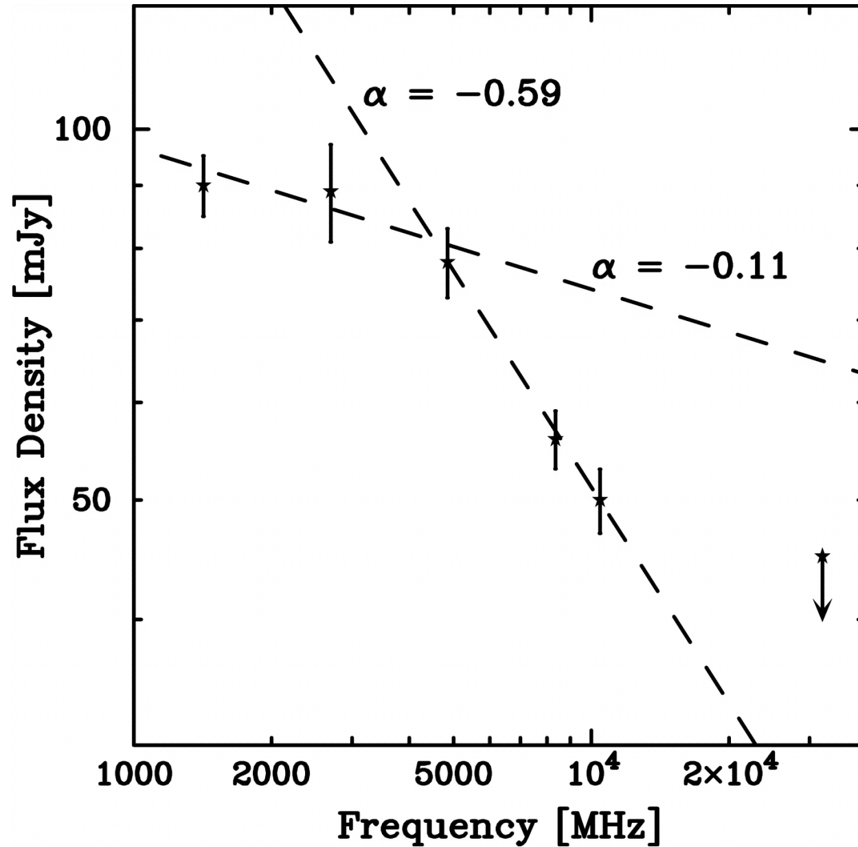
Fig. 3. from The Boomerang PWN G106.6+2.9 and the Magnetic Field Structure in Pulsar Wind Nebulae Kothes, Reich, & Uyanker 2006 ApJ 638 225 doi:10.1086/498666 https://dx.doi.org/10.1086/498666 © 2006. The American Astronomical Society. All rights reserved. Printed in U.S.A.
