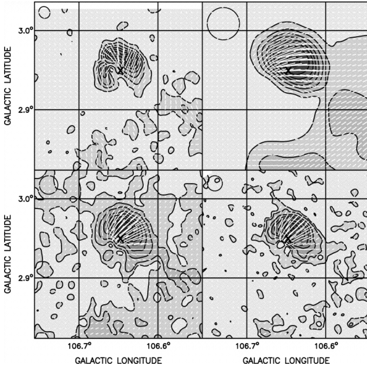
Fig. 2. from The Boomerang PWN G106.6+2.9 and the Magnetic Field Structure in Pulsar Wind Nebulae Kothes, Reich, & Uyankar 2006 ApJ 638 225 doi:10.1086/498666 https://dx.doi.org/10.1086/498666
