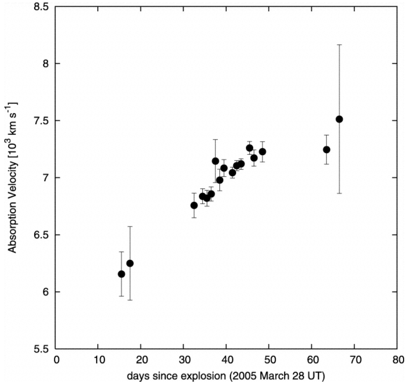
Fig. 3. from The Unique Type Ib Supernova 2005bf: A WN Star Explosion Model for Peculiar Light Curves and Spectra Tominaga et al. 2005 ApJL 633 L97 doi:10.1086/498570 https://dx.doi.org/10.1086/498570
