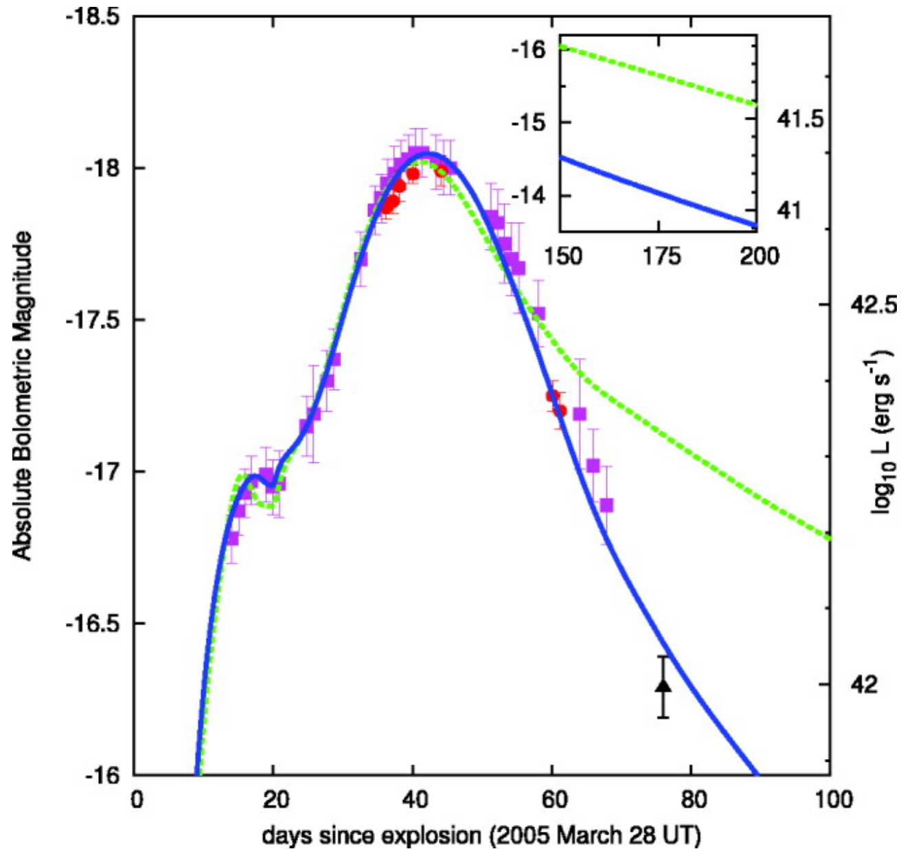
Fig. 2. from The Unique Type Ib Supernova 2005bf: A WN Star Explosion Model for Peculiar Light Curves and Spectra Tominaga et al. 2005 ApJL 633 L97 doi:10.1086/498570 https://dx.doi.org/10.1086/498570
