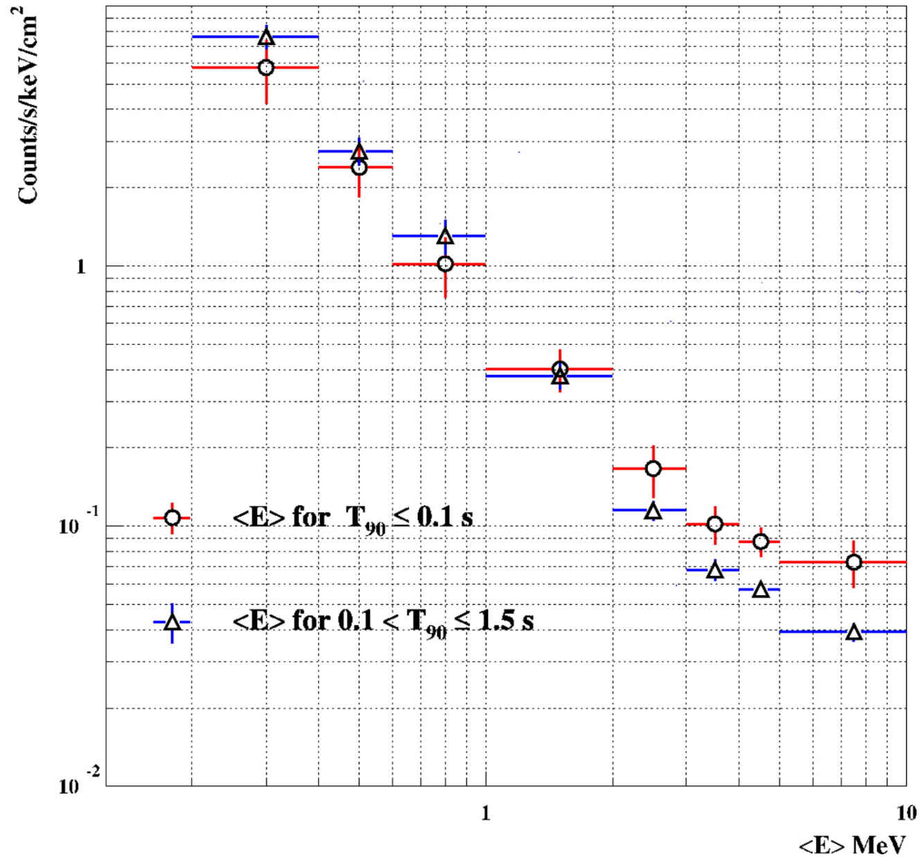
Fig. 4. from Study of Very Short GammaRay Bursts: New Results from BATSE and Konus Cline et al. 2005 ApJL 633 L73 doi:10.1086/498567 https://dx.doi.org/10.1086/498567 © 2005. The American Astronomical Society. All rights reserved. Printed in U.S.A.
