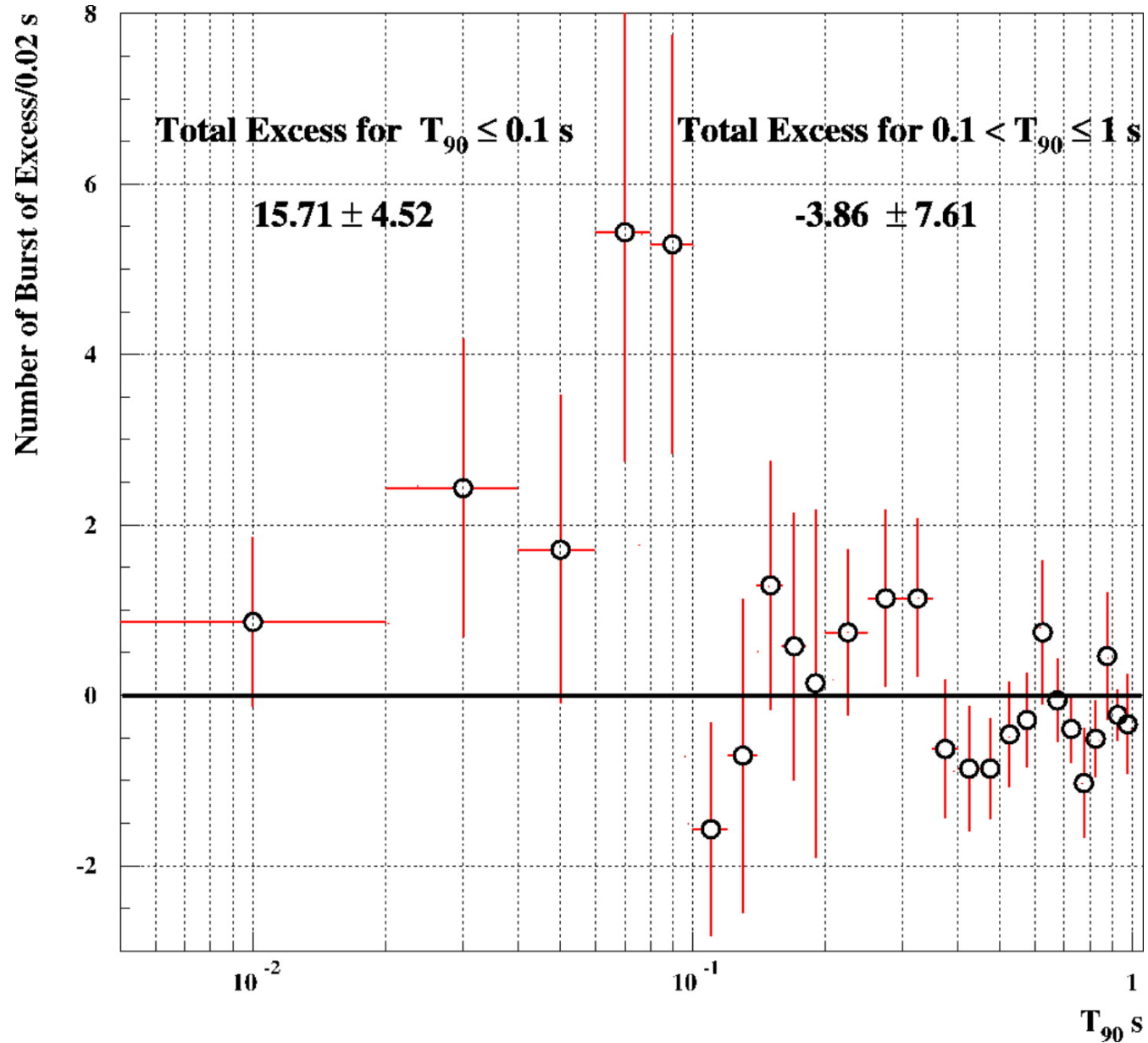
Fig. 2. from Study of Very Short GammaRay Bursts: New Results from BATSE and Konus Cline et al. 2005 ApJL 633 L73 doi:10.1086/498567 https://dx.doi.org/10.1086/498567
