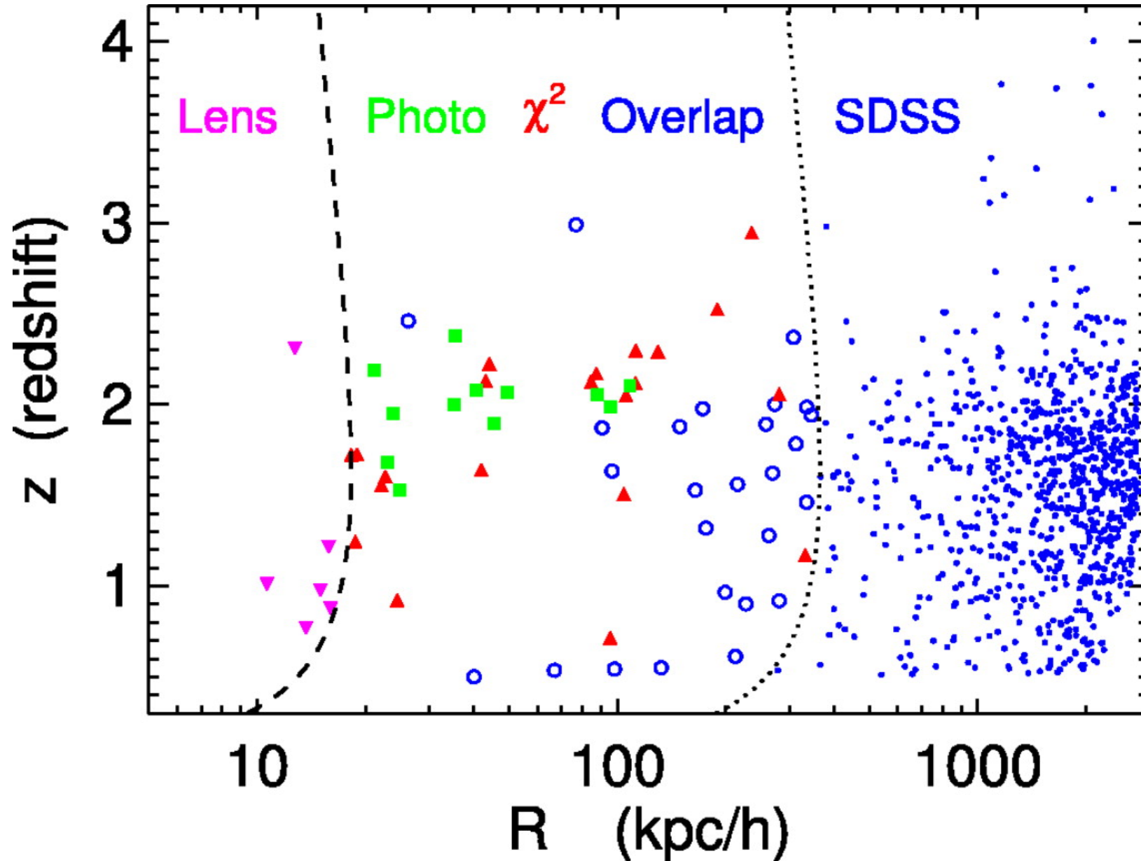
Fig. 3. from Binary Quasars in the Sloan Digital Sky Survey: Evidence for Excess Clustering on Small Scales Hennawi et al. 2006 AJ 131 1 doi:10.1086/498235 https://dx.doi.org/10.1086/498235 © 2006. The American Astronomical Society. All rights reserved. Printed in U.S.A.
