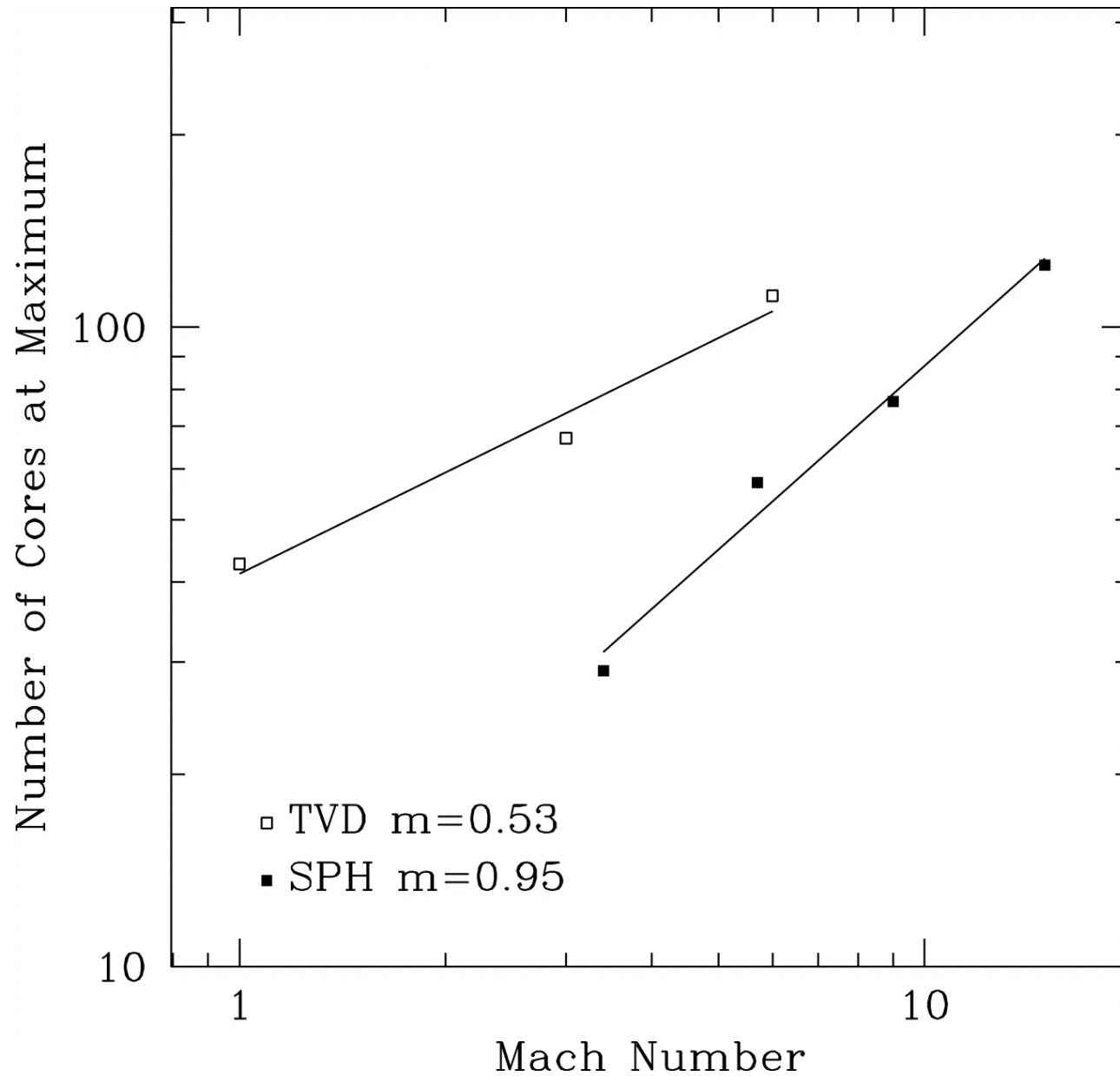
Fig. 6. from The Mass Spectra of Cores in Turbulent Molecular Clouds and Implications for the Initial Mass Function BallesterosParedes et al. 2006 ApJ 637 384 doi:10.1086/498228 https://dx.doi.org/10.1086/498228 © 2006. The American Astronomical Society. All rights reserved. Printed in U.S.A.
