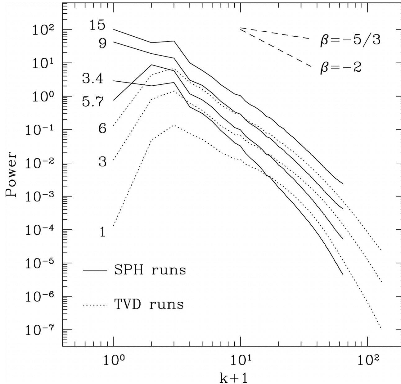
Fig. 2. from The Mass Spectra of Cores in Turbulent Molecular Clouds and Implications for the Initial Mass Function BallesterosParedes et al. 2006 ApJ 637 384 doi:10.1086/498228 https://dx.doi.org/10.1086/498228 © 2006. The American Astronomical Society. All rights reserved. Printed in U.S.A.
