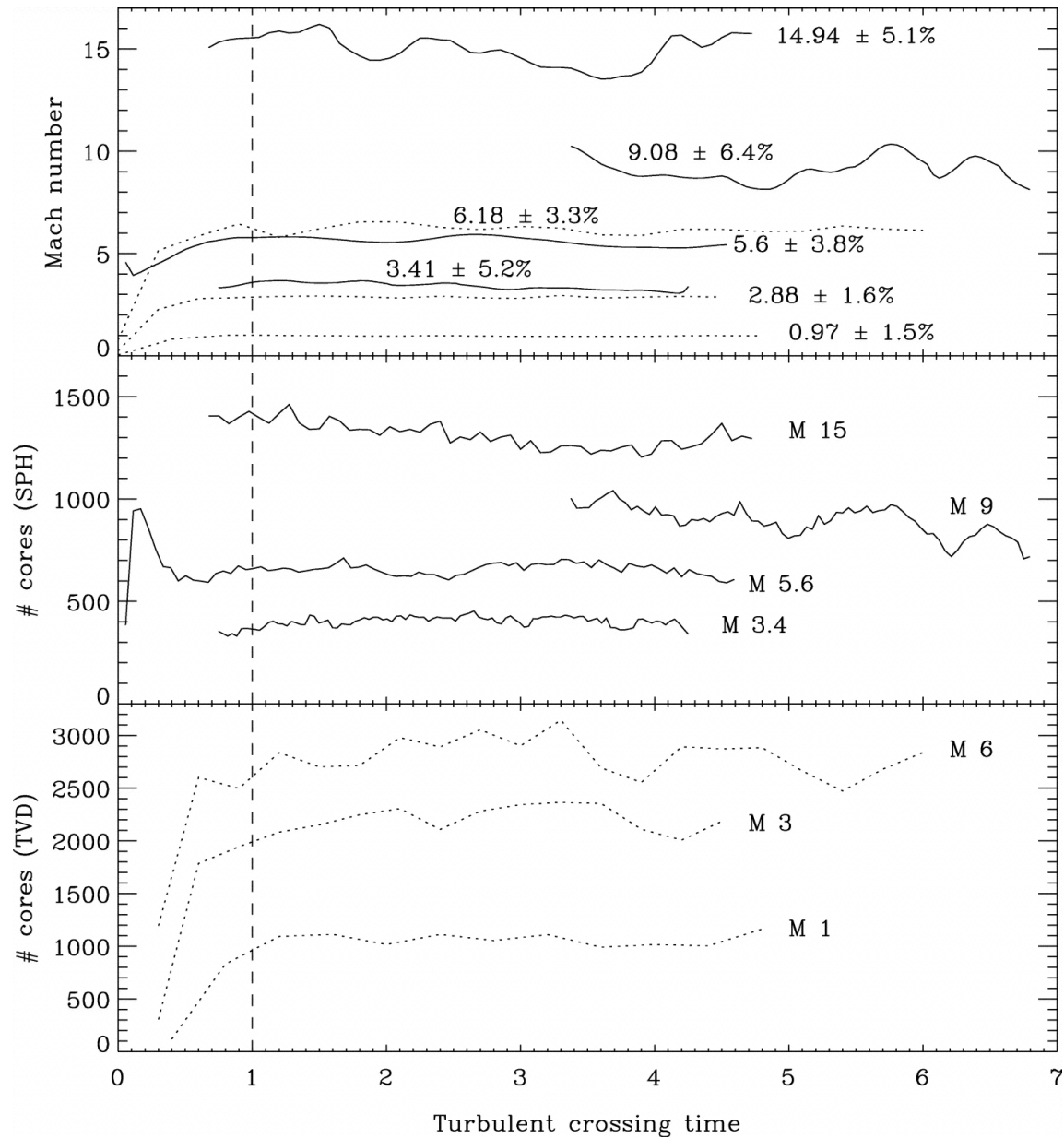
Fig. 1. from The Mass Spectra of Cores in Turbulent Molecular Clouds and Implications for the Initial Mass Function BallesterosParedes et al. 2006 ApJ 637 384 doi:10.1086/498228 https://dx.doi.org/10.1086/498228
