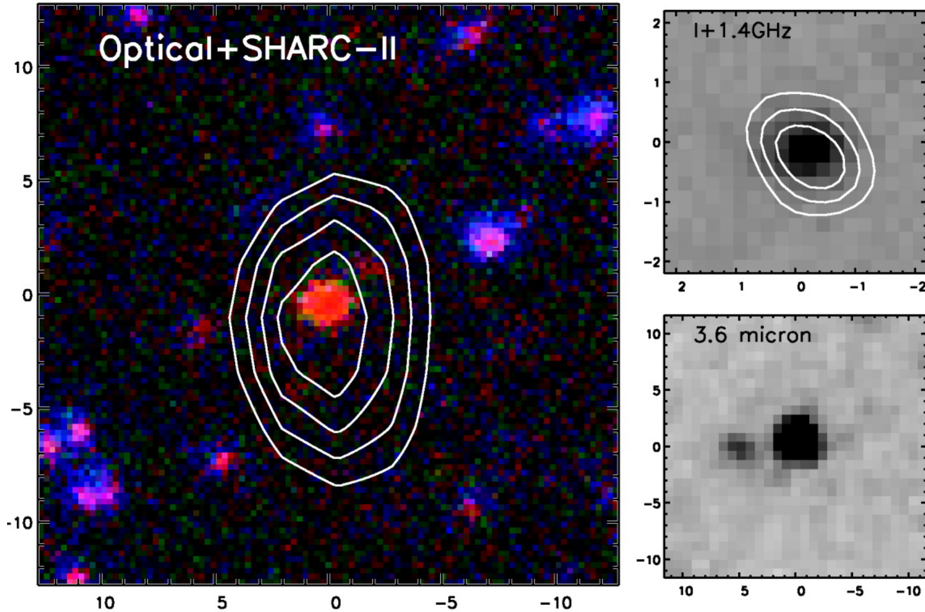
Fig. 1. from MIPS J142824.0+352619: A Hyperluminous Starburst Galaxy at z = 1.325 Borys et al. 2006 ApJ 636 134 doi:10.1086/497983 https://dx.doi.org/10.1086/497983 © 2006. The American Astronomical Society. All rights reserved. Printed in U.S.A.
