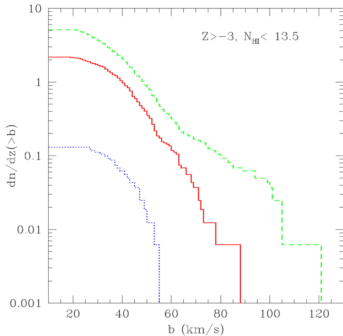
Fig. 9. from Quantitative Signatures of Galactic Superwinds on Ly Clouds and MetalLine Systems Cen, Nagamine, & Ostriker 2005 ApJ 635 86 doi:10.1086/497353 https://dx.doi.org/10.1086/497353 © 2005. The American Astronomical Society. All rights reserved. Printed in U.S.A.
